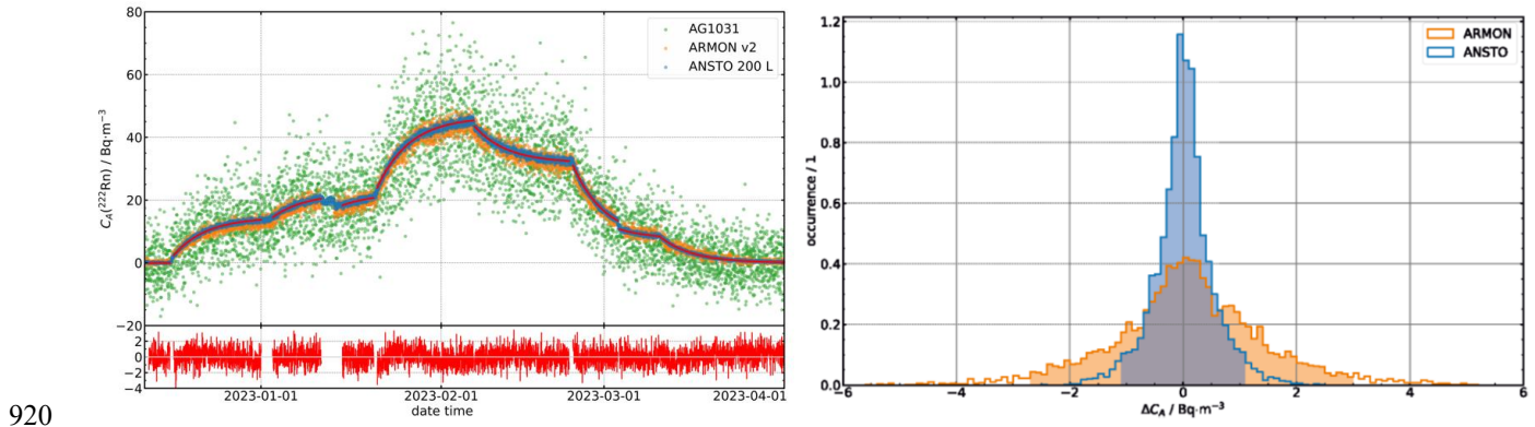
Figure 20: (a) 4-month comparison of the ANSTO 200 L and ARMON v2 monitors in the PTB climate chamber, and (b) comparison of standard deviations about the simulated chamber radon concentration (adapted from Röttger et al., 2025).
