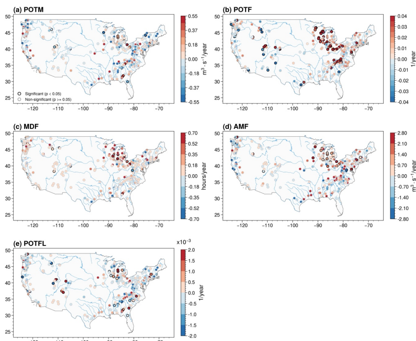
Figure 4. Trends in Peaks-over-threshold magnitude (POTM, a) , Peaks-over-threshold frequency (POTF, b) , mean duration of flood occurrence (MDF, c) , annual maximum flow (AMF, d) and Peaks-over-threshold flashiness (POTFL, e) . The color bar descriptions are consistent with those in Fig. 1.
