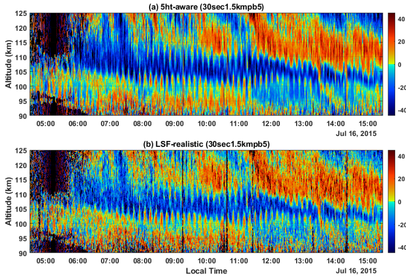
325 Figure 4. (a) Line-of-sight velocity derived from the 5ht-aware model (upper panel), (b) from the LSF-realistic method (lower panel). Positive velocity is away from the radar.
