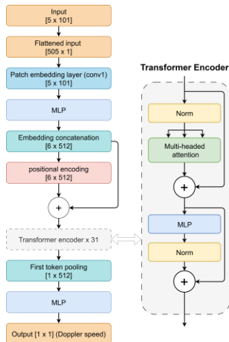
175 Figure 1. Model overview. The architecture consists of 31 transformer encoder blocks, 321 layers in total, and approximately 100 million parameters.
