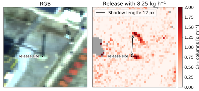
Figure 14. Left: RGB image of the study site with a marker on the release location at 6.5 m above ground. Right: \text{CH}_4 map of the study site with two plumes visible.
