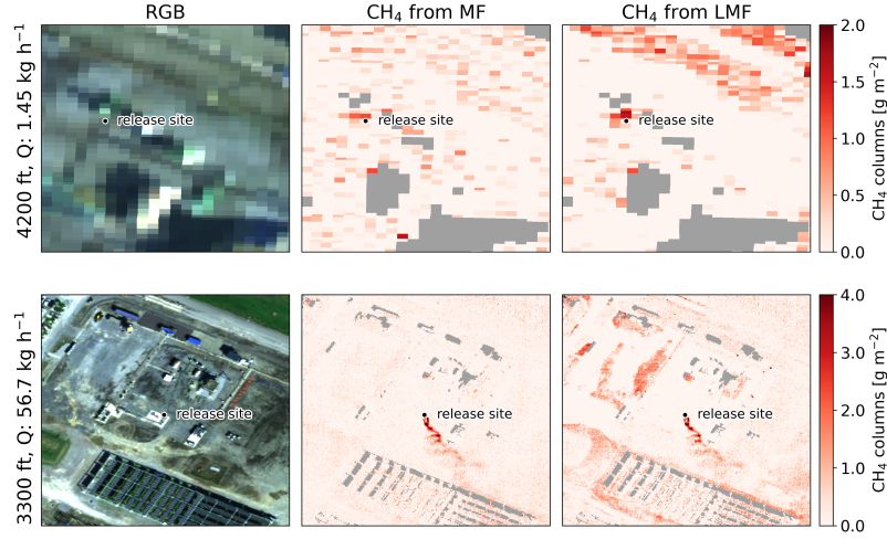
Figure 15. RGB images and \text{CH}_4 maps obtained from MF and LMF for release events with 1.45 and 56.7 \text{ kg CH}_4 \text{ h}^{-1} , observed at 4200 and 3300 ft. Note that the upper row shows a zoomed-in subsection of the scene to be able to see the short plume.
