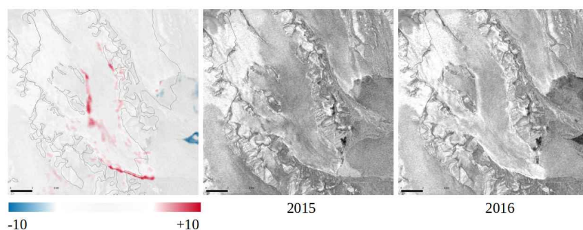
Figure 10: Example for detecting glacier surges from Radarsat-2 backscattering intensity change images for Wahlenbergreen. The change image in dB (left) is calculated as the ratio between the mosaics of winter backscatter intensity from 2016 (right) and 2015 (centre).
