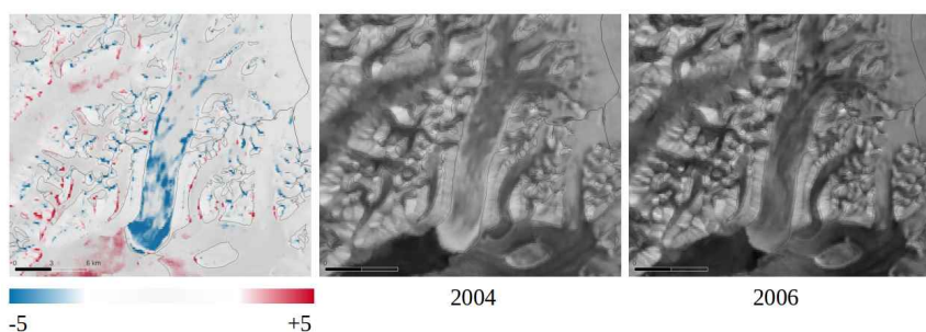
Figure 6: Example for detecting glacier surges from ENVISAT ASAR backscattering intensity change images for Tunabreen. The change image in dB (left) is calculated as the ratio between the mosaics of winter backscatter intensity from 2006 (right) and 2004 (centre).
