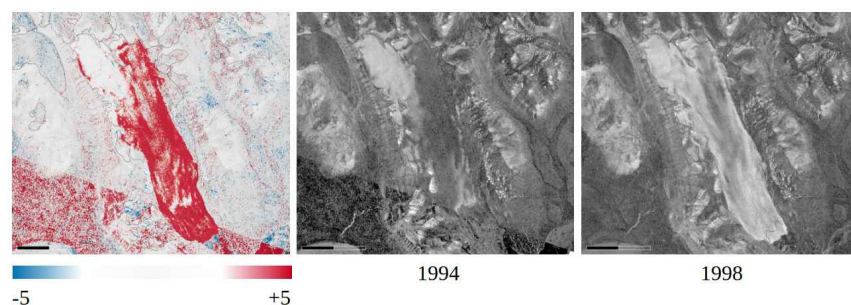
Figure 3: Example for detecting glacier surges from JERS-1 backscattering intensity change images for Fridtjovbreen. The change image in dB (left) is calculated as the ratio between the mosaics of winter backscatter intensity 1998 (right) and from 1994 (centre).
