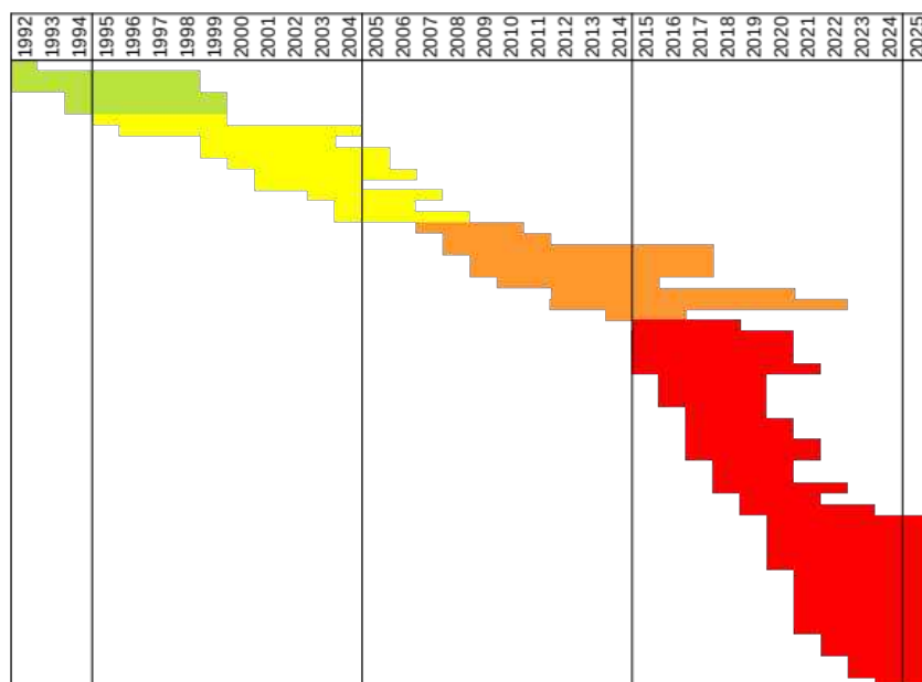
Figure 13: Surge events interpreted over Svalbard in the period 1992-2025 using ERS-1/2 SAR, JERS-1 SAR, ENVISAT ASAR, ALOS PALSAR, Radarsat-2 and Sentinel-1 data listed by start date. Green is before 1994, yellow is 1995-2005, orange is 2005-2014 and red is 2015-2025.
