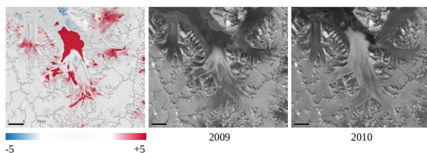
Figure 5: Example for detecting glacier surges from ENVISAT ASAR backscattering intensity change images for the Nathorstbreen glacier system, including Dobrowolskibreen, Polakkbreen and Zawadzkibreen. The change image in dB (left) is calculated as the ratio between the mosaics of winter backscatter intensity from 2010 (right) and 2009 (centre).
