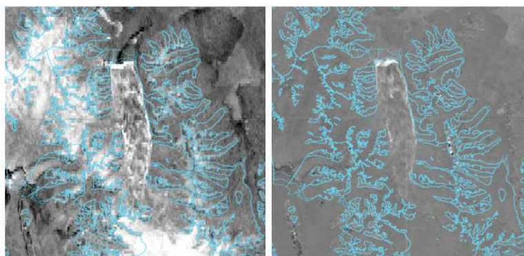
345 Figure 12: Left: example for detecting glacier surge from ALOS-2 PALSAR-2 annual backscattering intensity change images 2018-2019 for Monacobreen. Right: comparison to Sentinel-1 IW winter NDI images from maximum backscatter winter 2018 – winter 2019. Outlines from the Randolph Glacier Inventory 7.0 (RGI 7.0 Consortium, 2023) are shown in light blue.
