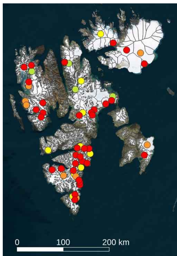
Figure 14: Surge events interpreted over Svalbard in the period 1992-2025 using ERS-1/2 SAR, JERS-1 SAR, ENVISAT ASAR, ALOS PALSAR, Radarsat-2 and Sentinel-1 data listed by start date. Green is before 1994, yellow is 1995-2005, orange is 2005-2014 and red is 2015-2025.
