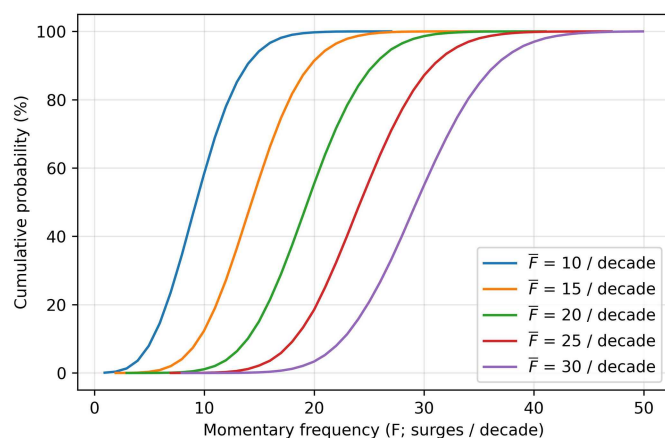
Figure 15: Cumulative probability functions of the momentary frequency of surge occurrence under different baseline surge frequencies due to constructive or destructive interference within the wide tested feature space, assuming that all surges have an independent (random) phase. The plots show that the probability of exceedence is directly tied to the baseline surge frequency; for example, more than 30 surges per decade will only consistently occur ( >10\% probability) with a baseline frequency of 20 surges per decade or more, and fewer than 10 will only consistently occur with a baseline of 15 surges per decade or less.
