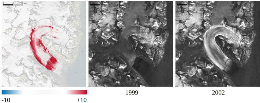
210 Figure 1: Example for detecting glacier surges from ERS-1/2 backscattering intensity change images for Ingerbreen. The change image in dB (left) is calculated as the ratio between the mosaics of winter backscatter intensity from 2002 (right) and 1999 (centre).
