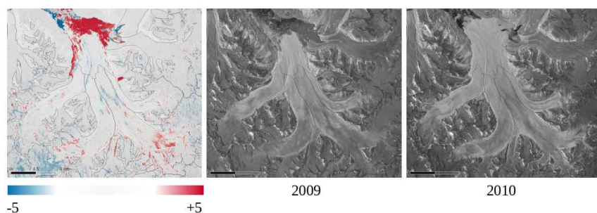
Figure 8: Example for detecting glacier surges from ALOS PALSAR backscattering intensity change images for the Nathorstbreen glacier system, including Dobrowolskibreen, Polakkbreen and Zawadzkbreen. The change image in dB (left) is calculated as the ratio between the mosaics of winter backscatter intensity from 2010 (right) and 2009 (centre).
