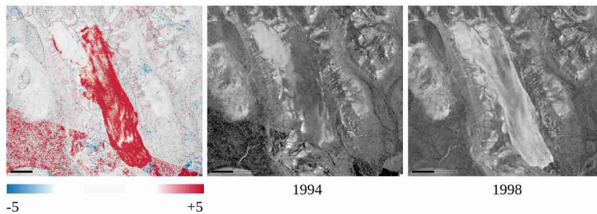
Figure 3: Example for detecting glacier surges from JERS-1 backscattering intensity change images for Fridtjovbreen. The change image in dB (left) is calculated as the ratio between the mosaics of winter backscatter intensity 1998 (right) and from 1994 (centre).
