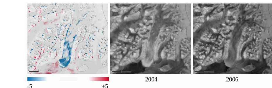
Figure 6: Example for detecting glacier surges from ENVISAT ASAR backscattering intensity change images for Tunabreen. The change image in dB (left) is calculated as the ratio between the mosaics of winter backscatter intensity from 2006 (right) and 2004 (centre).
