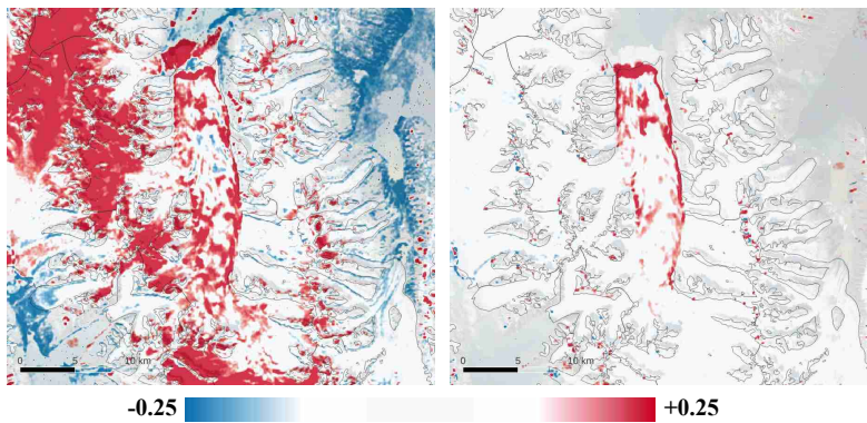
Figure 12: Left: example for detecting glacier surge from ALOS-2 PALSAR-2 normalized annual backscattering intensity change images 2017-2018 for Monacobreen. Right: comparison to Sentinel-1 IW winter NDI images from maximum backscatter winter 2018 – winter 2019. Outlines from the Randolph Glacier Inventory 7.0 (RGI 7.0 Consortium, 2023) are shown in black.
