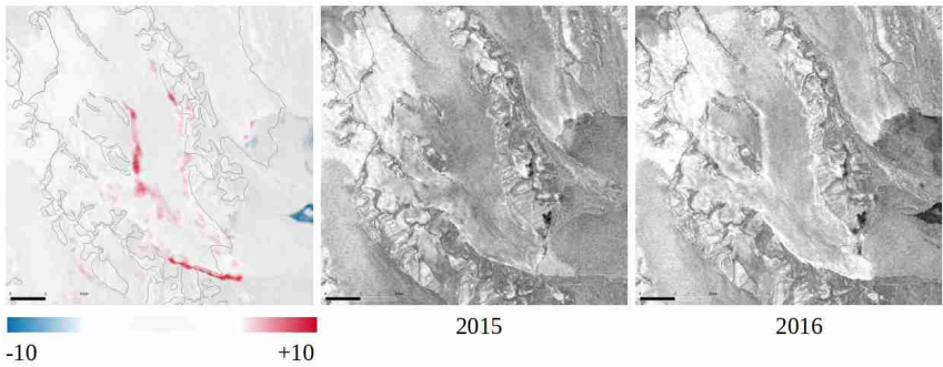
320 Figure 10: Example for detecting glacier surges from Radarsat-2 backscattering intensity change images for Wahlenbergbreen. The change image in dB (left) is calculated as the ratio between the mosaics of winter backscatter intensity from 2016 (right) and 2015 (centre).
