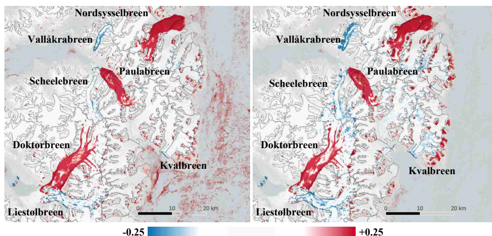
Figure 11: Example for detecting glacier surges from Sentinel-1 NDI images from maximum backscatter winter 2024 – winter 2025 computed from IW (left) and EW (right) data for (from south-west to north-east) Liestølbreen, Doktorbreen, Scheelebreen, Vallåkrabreen, Paulabreen, Nordsysselbreen and Kvalbreen. Outlines from the Randolph Glacier Inventory 7.0 (RGI 7.0 Consortium, 2023) are shown in black.
