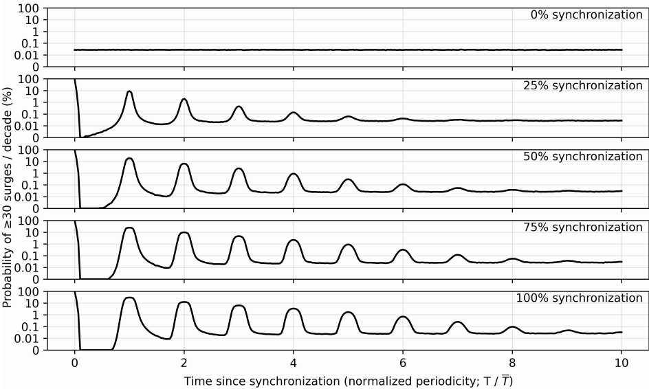
525 Figure 16: Exceedence probabilities of 30 surges per decade for the mean historical baseline surge frequency of 15 surges per decade within the wide tested feature space, tested over varying levels of phase synchronization. The plots reveal pulses of high momentary surge counts near the hypothetical synchronization event, before decorrelating to the baseline frequency over a number of average return period lengths. The analysis supports that many surges at once is much more easy to explain if some level of phase synchronization is introduced.
