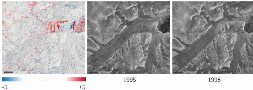
Figure 4: Example for detecting glacier surges from JERS-1 backscattering intensity change images for Chydeniusbreen. The change image in dB (left) is calculated as the ratio between the mosaics of winter backscatter intensity from 1998 (right) and 1995 (centre).
