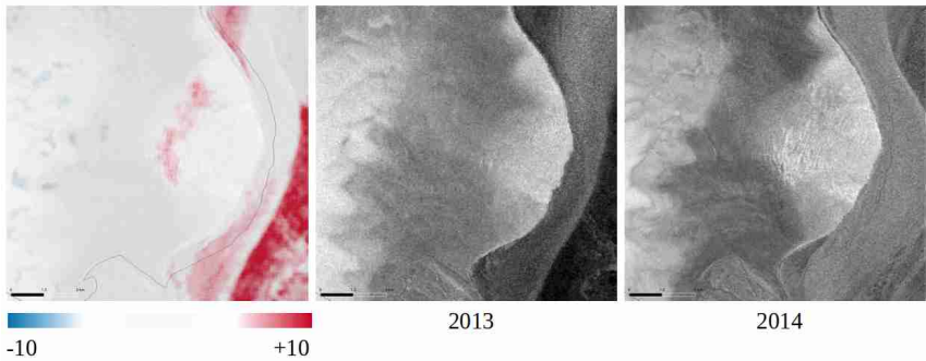
315 Figure 9: Example for detecting glacier surges from Radarsat-2 backscattering intensity change images for Stonebreen. The change image in dB (left) is calculated as the ratio between the mosaics of winter backscatter intensity from 2014 (right) and 2013 (centre). Outlines from the Randolph Glacier Inventory 7.0 (RGI 7.0 Consortium, 2023) are shown in black; backscatter changes off the glacier are related to differences in sea ice conditions.
