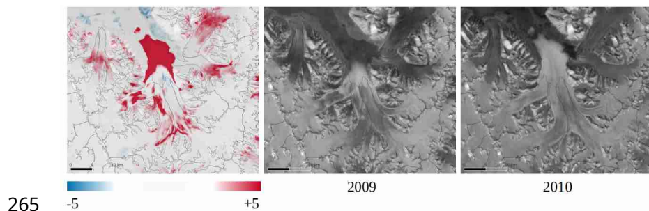
Figure 5: Example for detecting glacier surges from ENVISAT ASAR backscattering intensity change images for the Nathorstbreen glacier system, including Dobrowolskibreen, Polakkbreen and Zawadzkibreen. The change image in dB (left) is calculated as the ratio between the mosaics of winter backscatter intensity from 2010 (right) and 2009 (centre).
