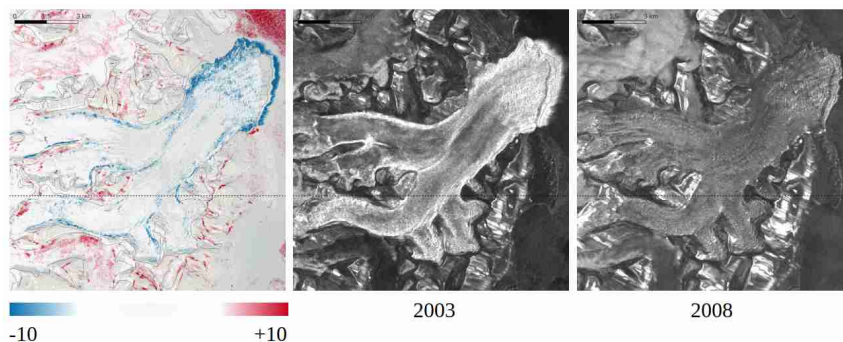
Figure 2: Example for detecting glacier surges from ERS-1/2 backscattering intensity change images for Perseibreen. The change image in dB (left) is calculated as the ratio between the mosaics of winter backscatter intensity from 2008 (right) and 2003 (centre).
