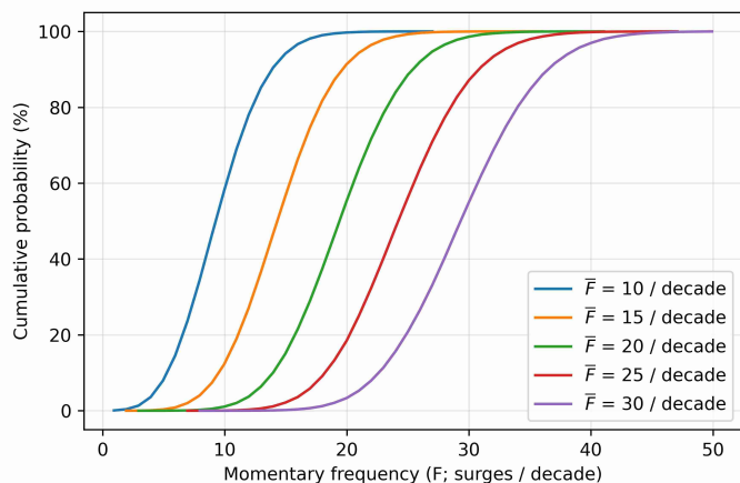
500 Figure 15: Cumulative probability functions of the momentary frequency of surge occurrence under different baseline surge frequencies due to constructive or destructive interference within the wide tested feature space, assuming that all surges have an independent (random) phase. The plots show that the probability of exceedence is directly tied to the baseline surge frequency; for example, more than 30 surges per decade will only consistently occur ( >10\% probability) with a baseline frequency of 20 surges per decade or more, and fewer than 10 will only consistently occur with a baseline of 15 surges per decade or less.
