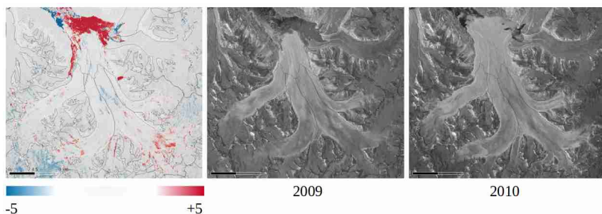
Figure 8: Example for detecting glacier surges from ALOS PALSAR backscattering intensity change images for the Nathorstbreen glacier system, including Dobrowolskibreen, Polakkbreen and Zawadzkiibreen. The change image in dB (left) is calculated as the ratio between the mosaics of winter backscatter intensity from 2010 (right) and 2009 (centre).
