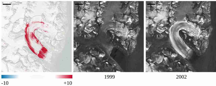
Figure 1: Example for detecting glacier surges from ERS-1/2 backscattering intensity change images for Ingerbreen. The change image in dB (left) is calculated as the ratio between the mosaics of winter backscatter intensity from 2002 (right) and 1999 (centre).
