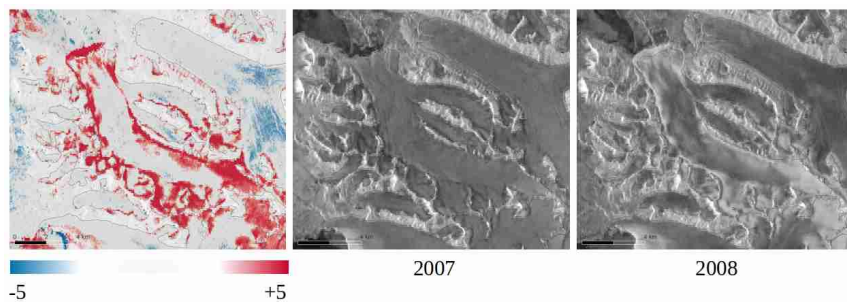
Figure 7: Example for detecting glacier surges from ALOS PALSAR backscattering intensity change images for Comfortlessbreen. The change image in dB (left) is calculated as the ratio between the mosaics of yearly backscatter intensity from 2008 (right) and 2007 (centre).
