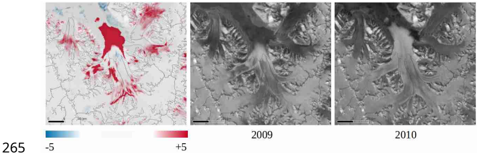
Figure 5: Example for detecting glacier surges from ENVISAT ASAR backscattering intensity change images for the Nathorstbreen glacier system, including Dobrowolskibreen, Polakkbreen and Zawadzkibreen. The change image in dB (left) is calculated as the ratio between the mosaics of winter backscatter intensity from 2010 (right) and 2009 (centre).
