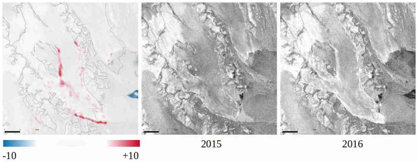
Figure 10: Example for detecting glacier surges from Radarsat-2 backscattering intensity change images for Wahlenbergbreen. The change image in dB (left) is calculated as the ratio between the mosaics of winter backscatter intensity from 2016 (right) and 2015 (centre).
