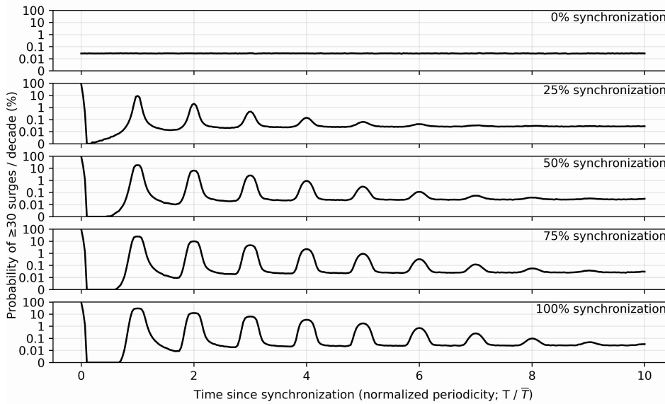
Figure 16: Exceedence probabilities of 30 surges per decade for the mean historical baseline surge frequency of 15 surges per decade within the wide tested feature space, tested over varying levels of phase synchronization. The plots reveal pulses of high momentary surge counts near the hypothetical synchronization event, before decorrelating to the baseline frequency over a number of average return period lengths. The analysis supports that many surges at once is much more easy to explain if some level of phase synchronization is introduced.
