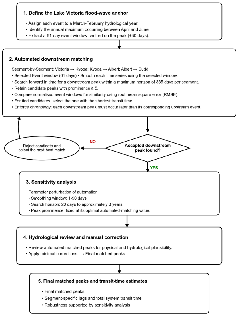
270 Fig 2: Schematic workflow of the automated floodwave tracking framework used to estimate system transit times. The process includes identification of Lake Victoria anchor events, automated downstream peak matching across the Victoria–Kyoga–Albert–Sudd cascade, sensitivity analysis of matching parameters, and final manual verification before estimation of segment and system-scale transit times.
