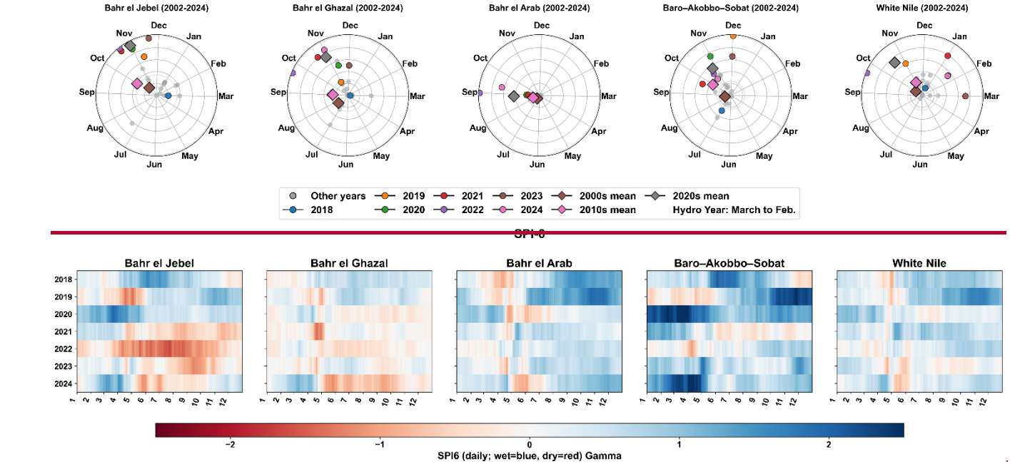
Fig. 4: Seasonality of annual maxima (top panels) and rainfall anomalies (bottom panels) for the South Sudan sub-catchments based on MODIS wetland extent and SPI-6 rainfall indices. The top panels show the timing of annual wetland-extent maxima for Bahr el Jebel, Bahr el Ghazal, Bahr el Arab, Baro Akobbo Sobat, and the White Nile during 2002–2024, grouped by decade and referenced to the hydrological year (March–February). The lower panels present six-month Standardized Precipitation Index (SPI-6) anomalies for 2018–2024 relative to the 1983–2017 climatology. The palette (wet = blue, dry = red) follows standard SPI categories: severely
