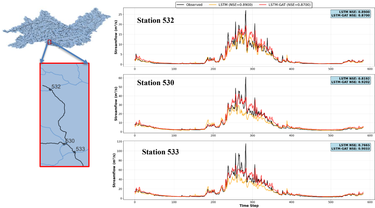
355 Figure 9: Hydrograph comparisons between LSTM and LSTM-GAT models at Matreier Tauernhaus (Station 532), Waier (Station 530), and Bruehl (Station 533) on the Isel River system.
