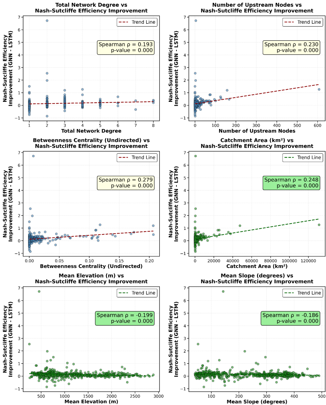
295 Figure 7: Relationship between performance improvement ( \Delta NSE) and static catchment attributes. Each panel shows scatter plots with Spearman's rank correlation coefficient ( \rho ) and significance levels. Positive \Delta NSE values indicate stations where LSTM-GAT outperformed the baseline LSTM model
