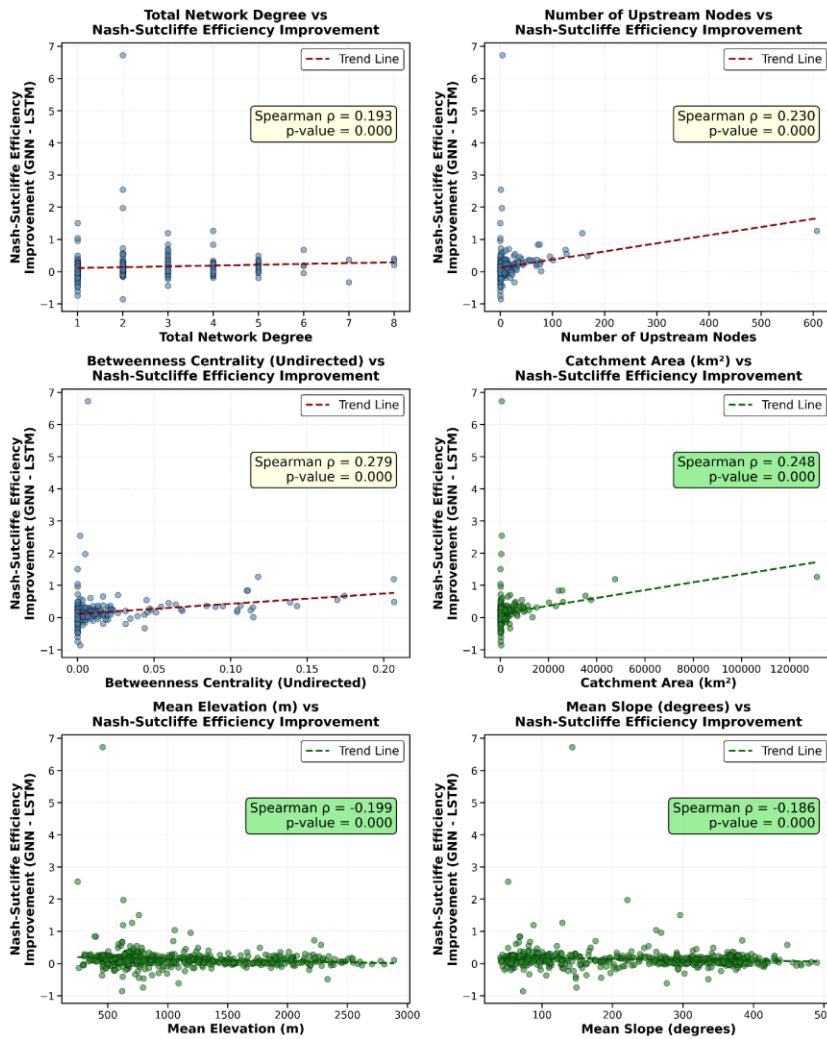
Figure 7: Relationship between performance improvement (ANSE) and static catchment attributes. Each panel shows scatter plots with Spearman's rank correlation coefficient ( \rho ) and significance levels. Positive ANSE values indicate stations where LSTM-GAT outperformed the baseline LSTM model
