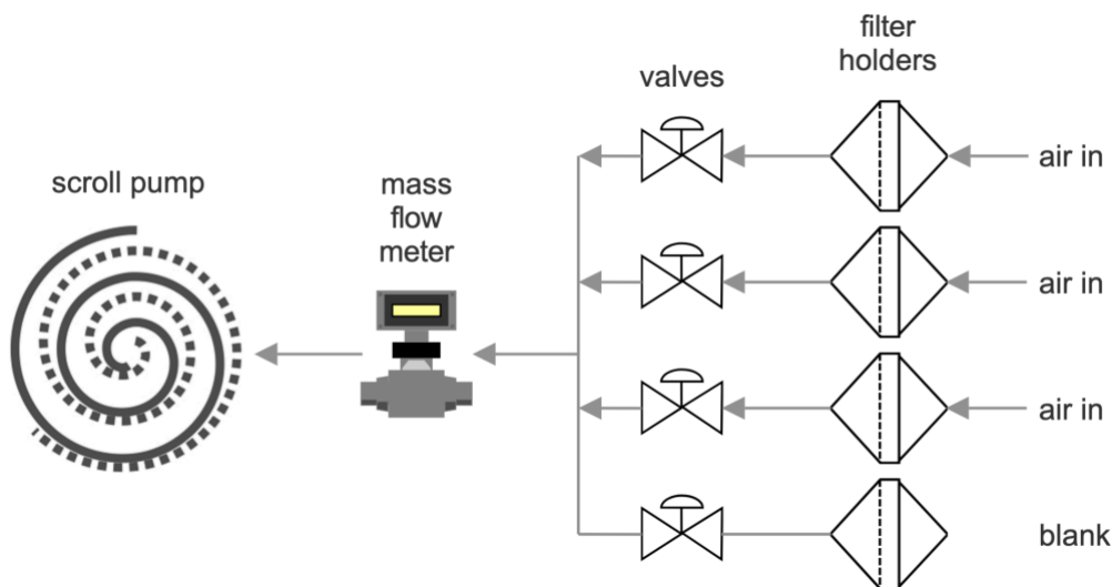
138 139 Figure 1: Schematic of PUFIN airflow. Main components are labeled. Valves are sequentially triggered to direct airflow through one filter 140 at a time, while the fourth filter serves as a field blank and remains closed to airflow. Arrows indicate direction of airflow. The schematic 141 was generated with SmartDraw.com.
