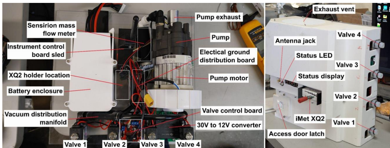
168 Figure 3: Photos of the interior (left) and immediate exterior (right) of PUFIN. The main components and features are labeled. The exterior 169 housing shown in the right image is 3D printed. 170
