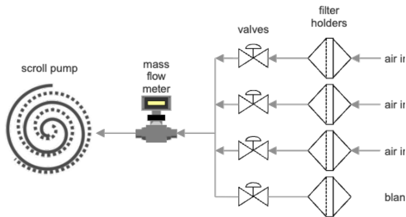
132 133 Figure 1: Schematic of PUFIN airflow. Main components are labeled. Valves are sequentially triggered to direct airflow through one filter 134 at a time, while the fourth filter serves as a field blank and remains closed to airflow. Arrows indicate direction of airflow. The schematic 135 was generated with SmartDraw.com.
