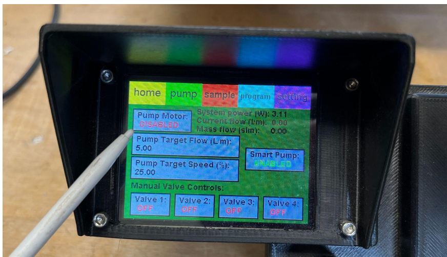
206 Figure 4: Photo of the PUFIN ground station undergoing manual operation. The image depicts the pump motor in an inactive state 207 ('DISABLED') with all four valves closed and 0 sL min -1 of flow. The target flow upon activation is 5.00 sL min -1 .
