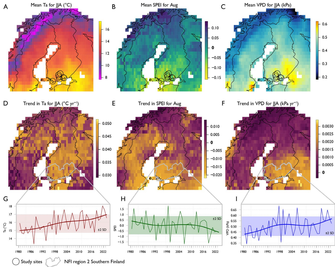
Figure 1. Regional climate and multi-decadal trends in southern Finland. Data based on CRU TS data (version 4.08) for the period 1980–2023. Panels show A) mean summer temperature ( T_a ) for June–August (JJA), B) mean August standardized precipitation–evapotranspiration index (SPEI), C) mean JJA vapor pressure deficit (VPD), D–F) Mann-Kendall trends in JJA T_a (°C yr -1 ), August SPEI (unitless yr -1 ), and JJA VPD (kPa yr -1 ), respectively. Circles in panels A–C) show the location of the study sites, while the polygon outlines in panels D–F) corresponds to the southern Finland region as defined by the Finnish NFI. Panels G–I) show the regional averaged time series (1980–2023) of T_a , SPEI, and VPD, with 30-year spline curves and the shaded area shows two standard deviations around the period mean.
