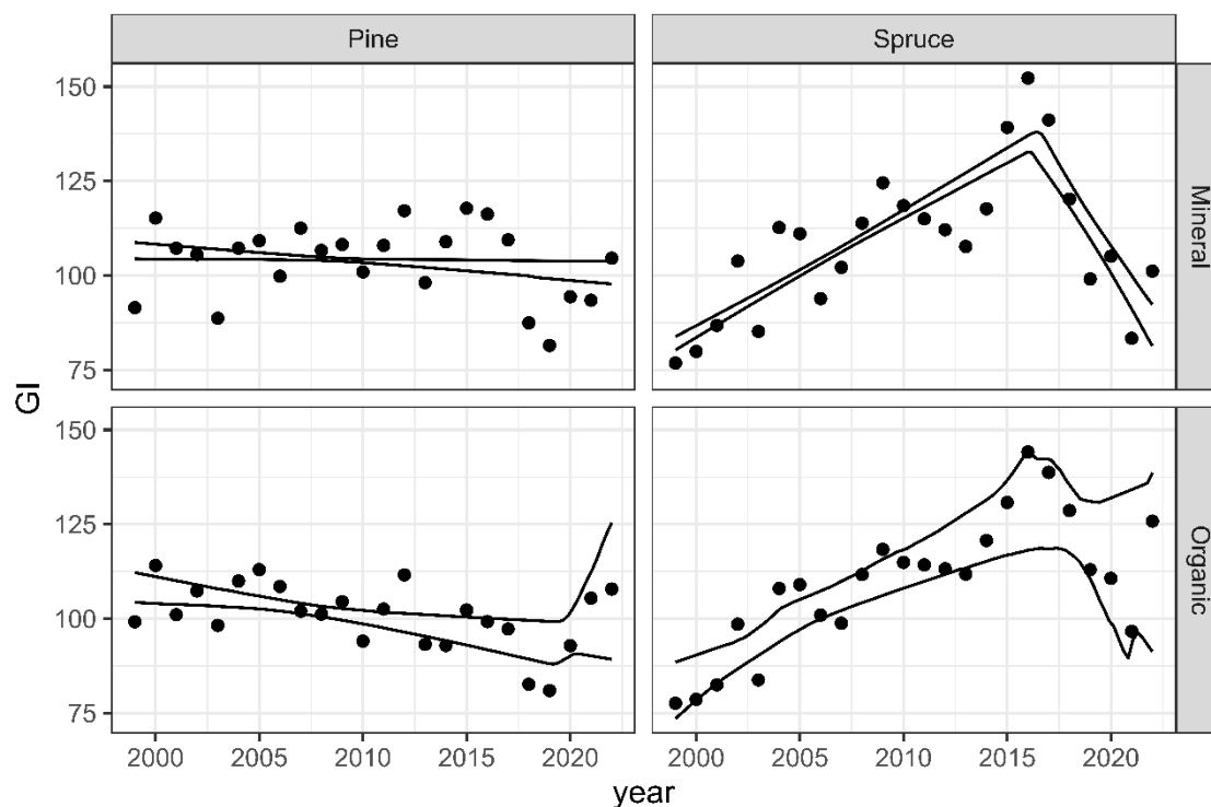
775 Figure A3. NFI-based standardized growth index (GI) and confidence intervals (95%) for segmented regression predictions, accounting for NFI sampling uncertainty. Points show GI; lines denote confidence intervals.
