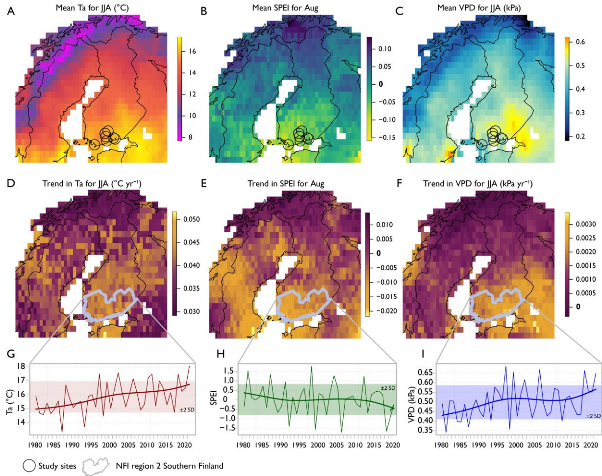
Figure 1. Regional climate and multi-decadal trends in southern Finland. Data based on CRU TS data (version 4.08) for the period 1980–2021. Panels show A) mean summer temperature (Ta) for June–August (JJA), B) mean August standardized precipitation–evapotranspiration index (SPEI), C) mean JJA vapor pressure deficit (VPD), D–F) Mann-Kendall trends in JJA Ta (°C yr -1 ), August SPEI (unitless yr -1 ), and JJA VPD (kPa yr -1 ), respectively. Circles in panels A–C) show the location of the study sites, while the polygon outlines in panels D–F) corresponds to the southern Finland region as defined by the Finnish NFI. Panels G–I) show the regional averaged time series (1980–2021) of Ta, SPEI, and VPD, with 30-year spline curves and the shaded area shows two standard deviations around the period mean.
