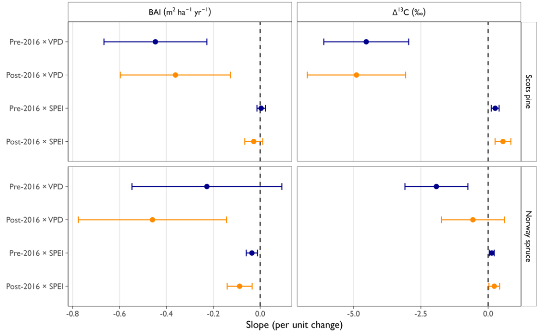
Figure 6. Sensitivity of basal area increment (BAI) and carbon isotope discrimination ( \Delta^{13}\text{C} ) to recent changes in water limitation. Standardized effect sizes (slopes \pm 95% confidence intervals) of summer (mean May–July SPEI and VPD) on annual tree ring BAI (A, C) and \Delta^{13}\text{C} (B, D) for Scots pine and Norway spruce respectively based on the LMM model runs described in Eq. (6). Blue and red points represent the pre-2016 (1990–2015 for BAI and 1999–2015 for \Delta^{13}\text{C} ) and post-2016 (2016–2023) periods, respectively, capturing shifts in climate sensitivity associated with recent intensified water limitation. Slopes indicate the estimated change in BAI ( \text{m}^2 \text{ha}^{-1} \text{yr}^{-1} ) and \Delta^{13}\text{C} (‰) per unit change in the respective climate variable. Error bars denote 95% confidence intervals. Effects are considered statistically significant when confidence intervals do not overlap zero.
