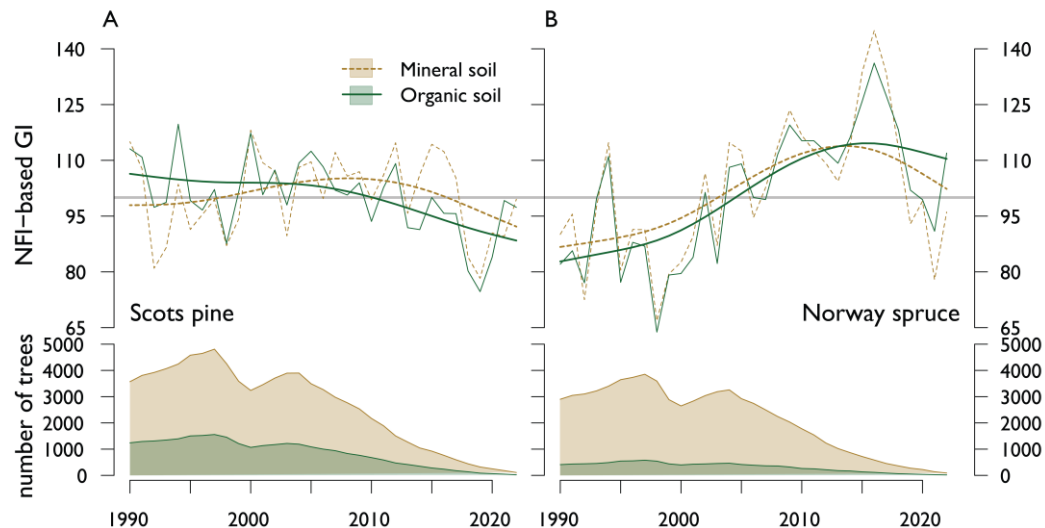
Figure 2. National Forest Inventory (NFI) based tree growth patterns in southern Finland. Panels show NFI-based standardized growth index (GI) for Scots pine (A) and Norway spruce (B) from 1990 to 2022 on mineral (red) and organic (green) soils. The upper panels illustrate the annual variability in GI for each tree species and soil type, with thin lines depicting the mean annual values, while thick lines showing the 30-year smoothing splines to illustrate long-term trends. The lower panels show the number of trees used to derive each annual GI estimate for each tree species and soil type (see Appendix A for NFI uncertainty estimates).
