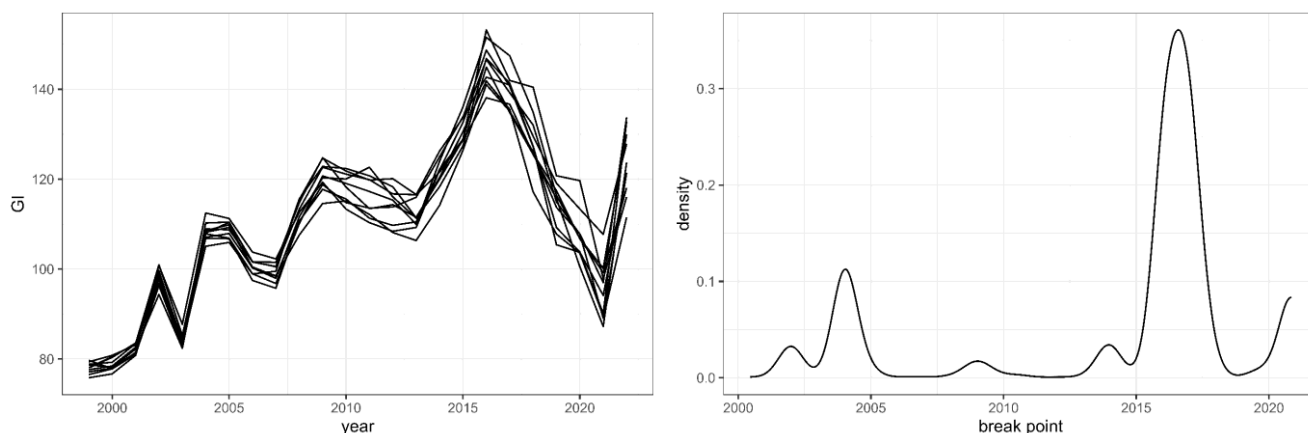
755 Figure A2. Left: Ten realisations of GI series for Norway spruce on organic soils, simulated from the distribution determined by the NFI sampling variance and correlations of the GI estimates. Right: Relative frequencies of all break points of segmented regression models fitted to the 1000 simulations from the uncertainty distribution of GIs for spruce on organic soils.
