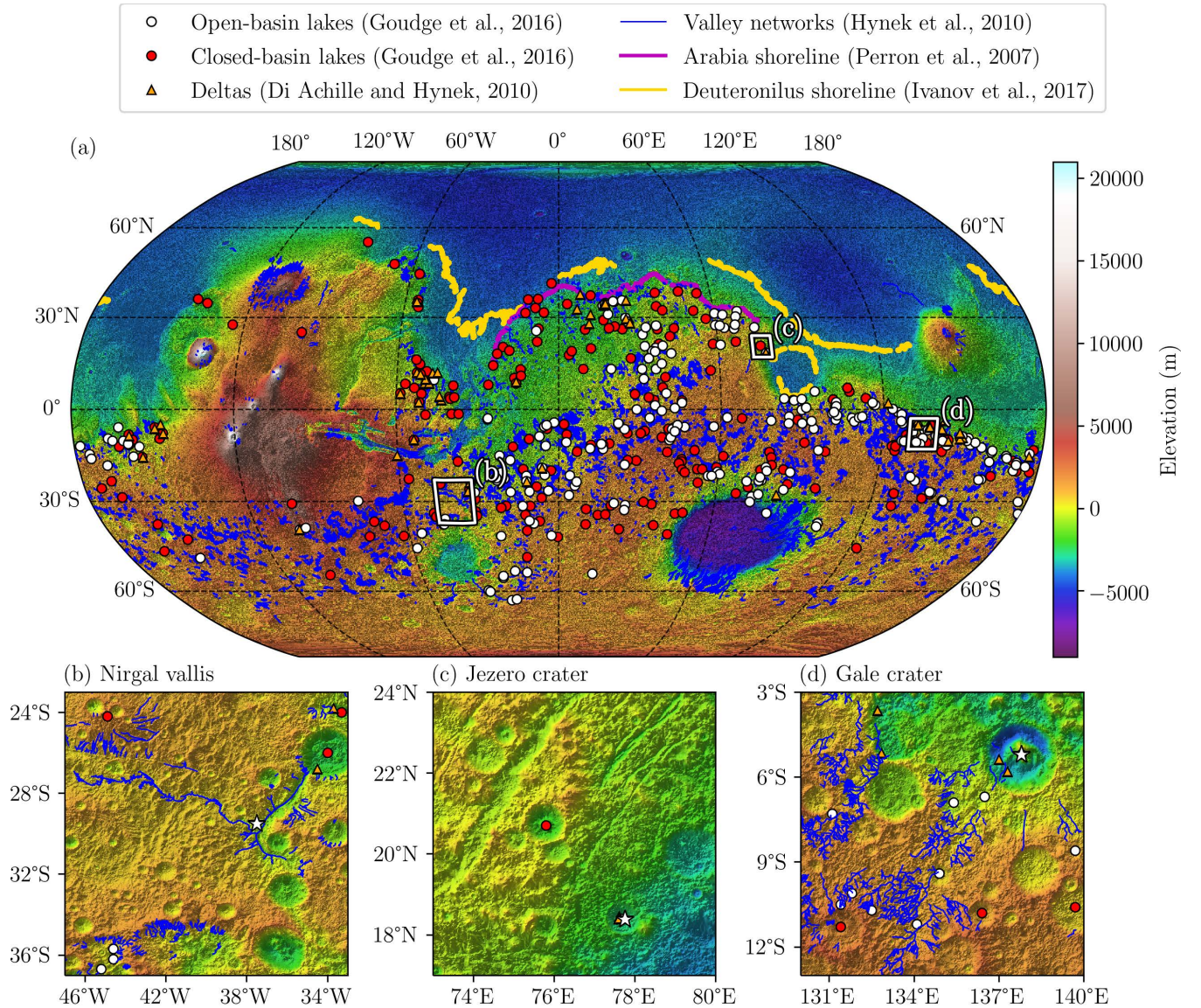
Figure 2. Mars topographic map showing the inventory of observed data relating to water flow effects. (a) Digital Elevation Model (DEM) from the Mars Orbiter Laser Altimeter (MOLA) (Smith et al., 2001; Neumann et al., 2001). The shaded relief is generated from the DEM with a sun angle of 45^\circ from horizontal and a sun azimuth of 315^\circ , as measured clockwise from north. The blue lines represent the valley networks (Hynek et al., 2010). The white and red dots represent open-basin and closed-basin lakes, respectively (Goudge et al., 2016). The orange triangles represent deltas (Di Achille and Hynek, 2010). The magenta and yellow lines represent respectively Arabia (Perron et al., 2007) and Deuteronilus (Ivanov et al., 2017) shorelines. The white squares are zoomed areas on Nirgal Vallis’ watershed (b), Jezero’ watershed (c) and Gale’ watershed (d). The white stars on the zoomed areas indicate the outlets of Nirgal Vallis (b), Jezero Crater (c), and Gale Crater (d).
