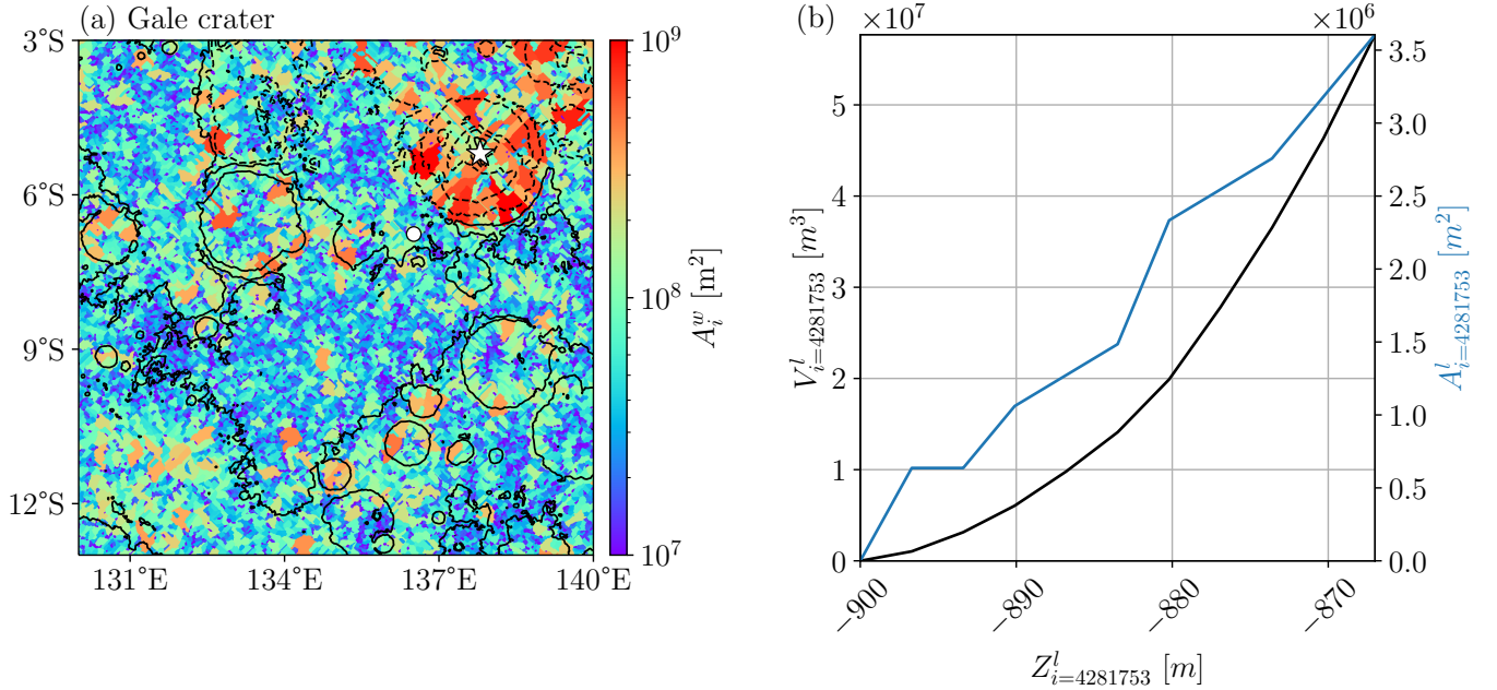
Figure 3. (a) 9,777 watersheds of leaf depressions are represented on the zoomed area of the Gale crater watershed (Figure 2d). Gale crater is localized by the white star. The color bar represents the watershed area A_i^w . (b) Example of pre-computed hydrological functions for a random depression ( i = 4281753 ) localized near to the Gale watershed by the white point (a). Evolution of the lake volume V_i^l (black line) and the lake area A_i^l (blue curve) as functions of the lake elevation Z_i^l .
