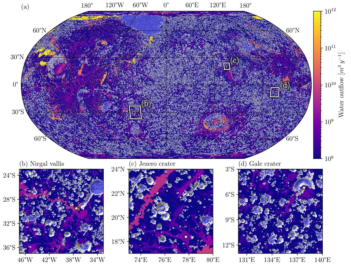
Figure D4. Water overflow at steady state with a GEL = 10 \text{ m} and E = 1 \text{ m.y}^{-1} . The color bar represents the water flow accumulation. The areas where there is no outflow are symbolized by white shaded areas and sky blue areas represent the watershed and lake/ocean areas. The first line of zoomed plots shows the raw output data of the hydrological model which represents the water overflow associated to the watershed area.
