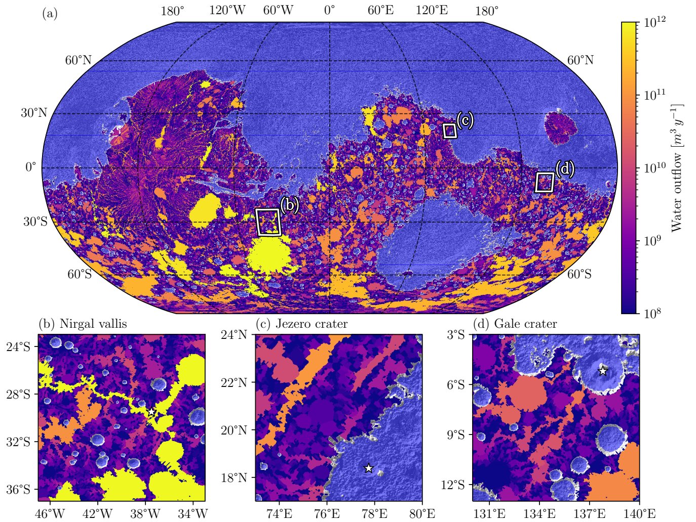
Figure D6. Water overflow at steady state with a GEL = 1,000 m and E = 1 m.y^{-1} . The color bar represents the water flow accumulation. The areas where there is no overflow are symbolized by white shaded areas and sky blue areas represent the watershed and lake/ocean areas. The first line of zoomed plots shows the raw output data of the hydrological model which represents the water overflow associated to the watershed area.
