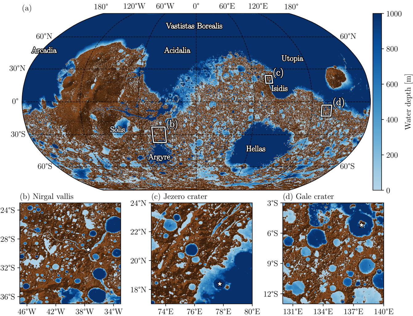
Figure D5. Distribution of water reservoirs (blue areas) at steady state with a GEL equal to 1,000 m. The color bar represents the water depth. The brown shaded areas represent the areas where the water cannot be accumulated. The white squares are zoomed areas on Nirgal Vallis' watershed (b), Jezero' watershed (c) and Gale' watershed (d). The white stars localized the Nirgal Vallis outlet (b), Jezero crater (c) and Gale crater (d).
