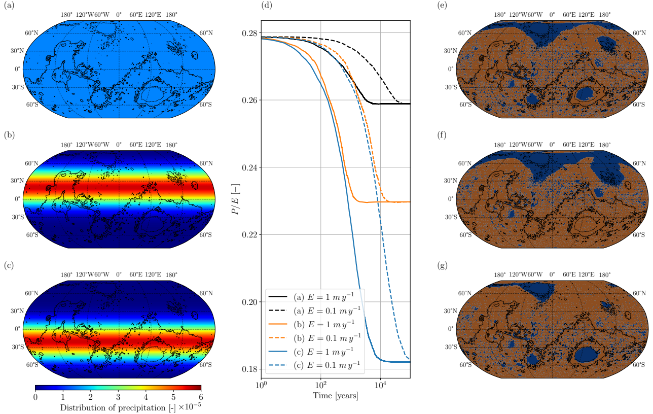
Figure C1. Simulations at steady state for a GEL = 100m with a varying precipitation pattern: (a) homogeneous precipitation pattern, (b) precipitation is concentrated around 20°N and (c) precipitation concentrated around 20°S. Simulations were performed with a degraded MOLA topography at 1 pixel per degree resolution. (d) Evolution of the ratio P/E for the three precipitation rate patterns and two homogeneous evaporation rate: 1 m/yr (solid curves) and 0.1 m/yr (dashed curves). Distribution of water reservoirs at steady state for the three precipitation patterns: (e) homogeneous precipitation pattern, (f) precipitation is concentrated around 20°N and (g) precipitation concentrated around 20°S.
