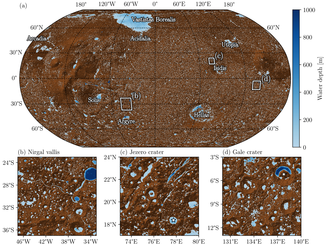
Figure D3. Distribution of water reservoirs (blue areas) at steady state with a GEL equal to 10 m. The color bar represents the water depth. The brown shaded areas represent the areas where the water cannot be accumulated. The white squares are zoomed areas on Nirgal Vallis' watershed (b), Jezero' watershed (c) and Gale' watershed (d). The white stars localized the Nirgal Vallis outlet (b), Jezero crater (c) and Gale crater (d).
