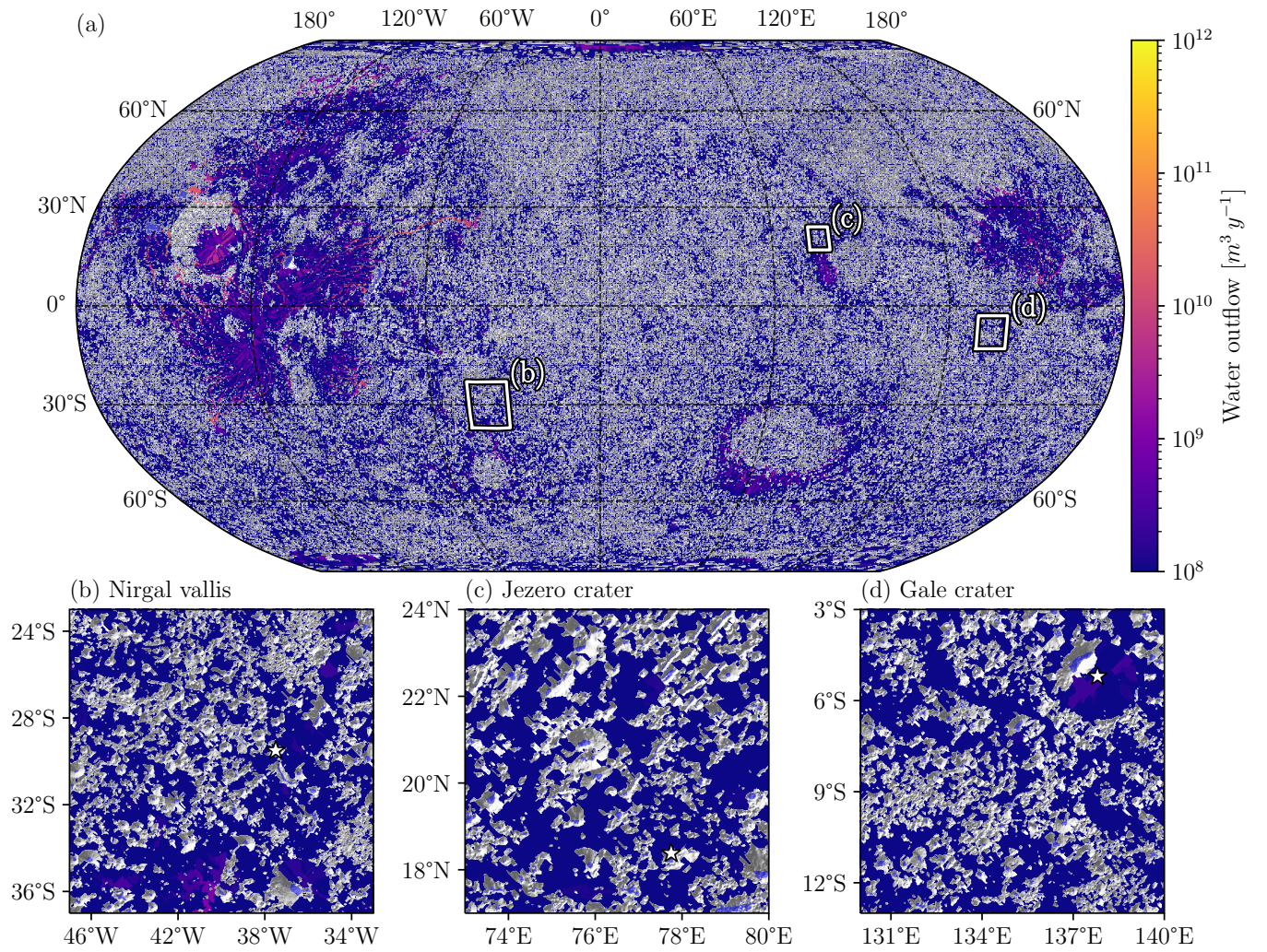
Figure D2. Water overflow at steady state with a GEL = 1\text{ m} and E = 1\text{ m.y}^{-1} . The color bar represents the water flow accumulation. The areas where there is no outflow are symbolized by white shaded areas and sky blue areas represent the watershed and lake/ocean areas. The first line of zoomed plots shows the raw output data of the hydrological model which represents the water overflow associated to the watershed area.
