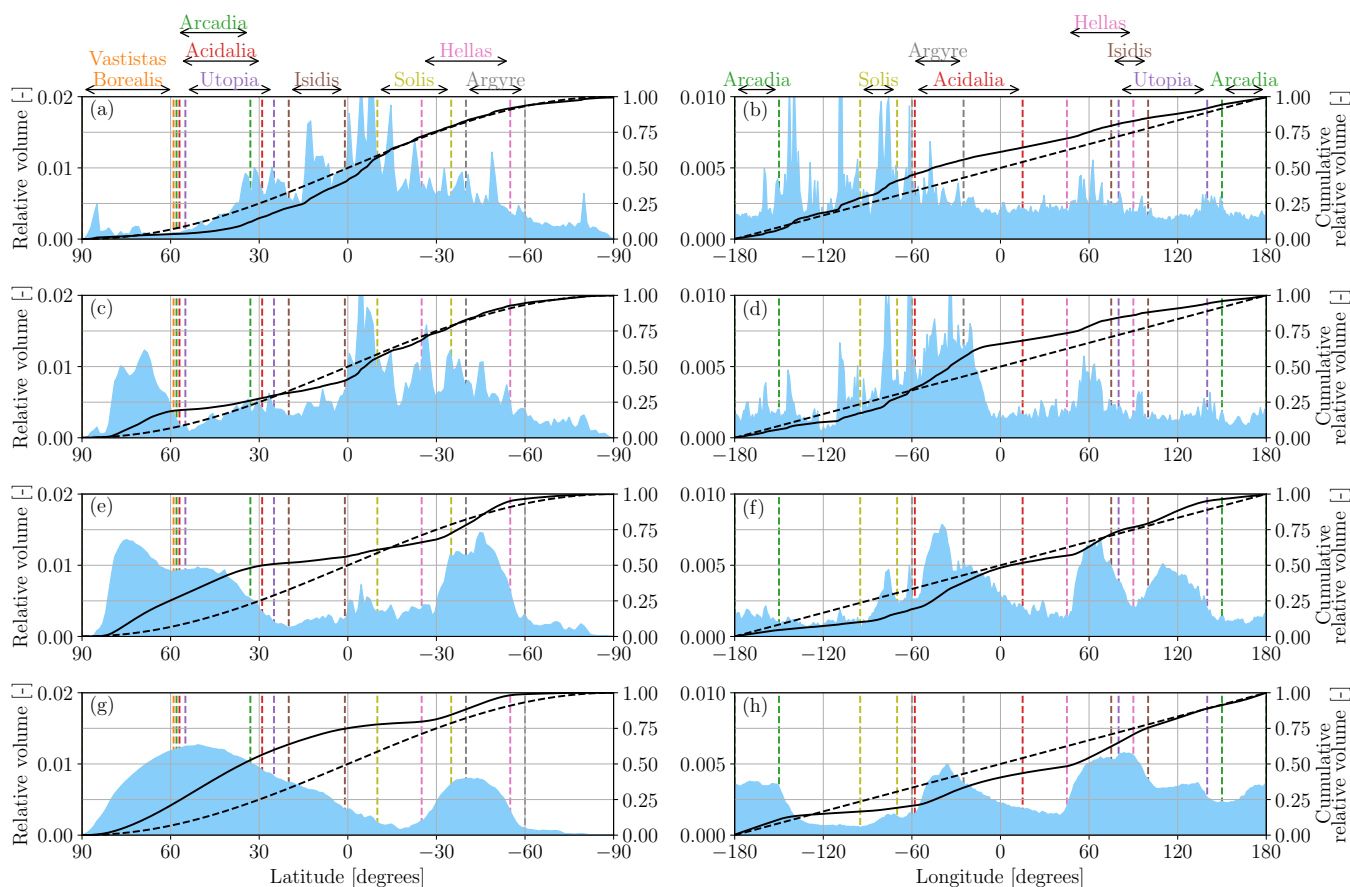
Figure 3. Distribution of water reservoirs at steady state for each GEL: 1 m (a, b), 10 m (c, d), 100 m (e, f), 1000 m (g, h). The blue areas represent the proportion of water relative to the total water volume (left y-axis) per degree of latitude (left column) and longitude (right column). The solid black lines show the cumulative relative water volume (right y-axis). The dashed black lines represent the cumulative relative water volume for a conceptual homogeneous distribution of water.
