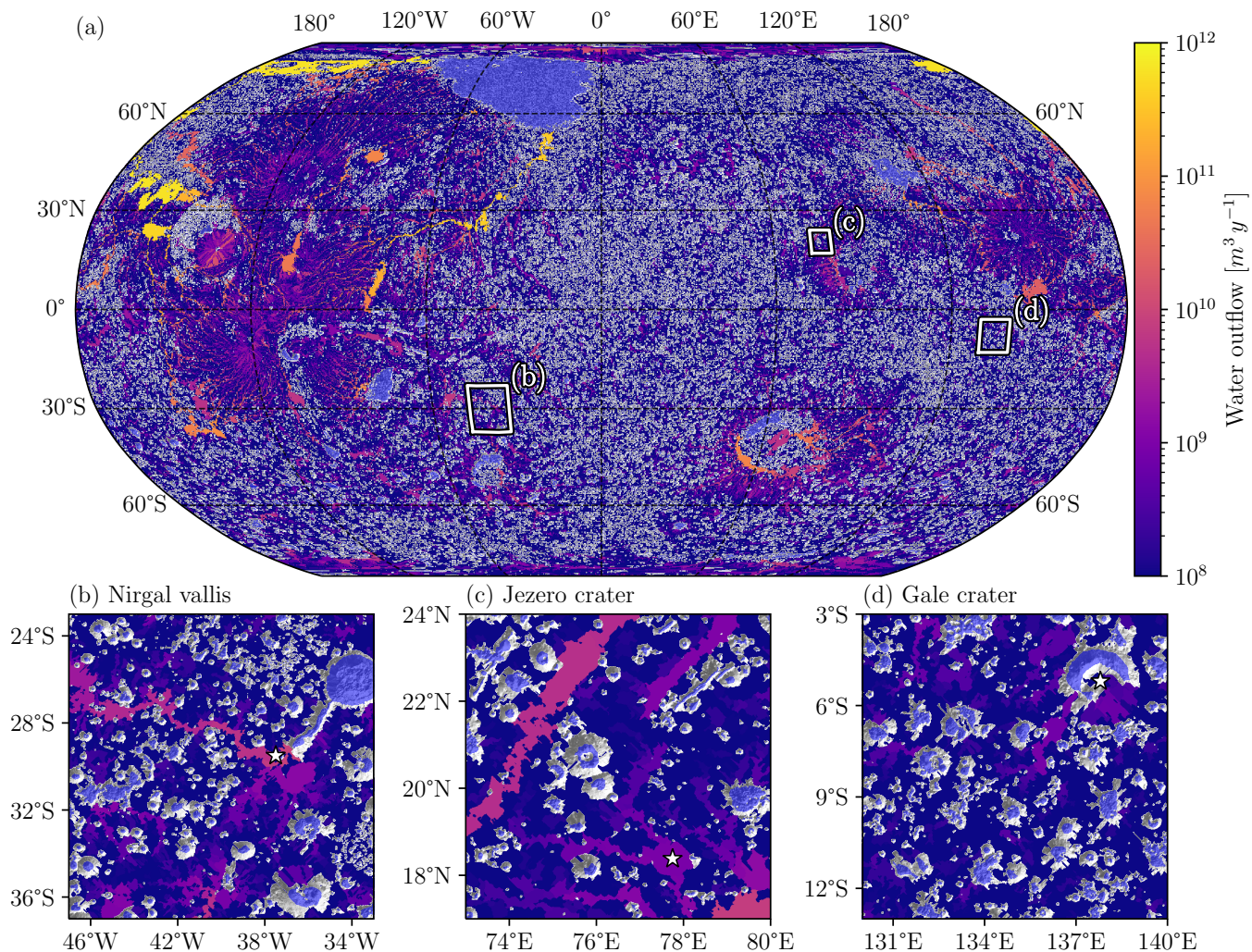
Figure B4. Water overflow at steady state with a GEL = 10 \text{ m} and E = 1 \text{ m.y}^{-1} . The color bar represents the water flow accumulation. The areas where there is no outflow are symbolized by white shaded areas and sky blue areas represent the watershed and lake/ocean areas. The first line of zoomed plots shows the raw output data of the hydrological model which represents the water overflow associated to the watershed area. The second line of zoomed plots shows the water overflow associated to the valley network, after post-processing explained in section 2.4.
