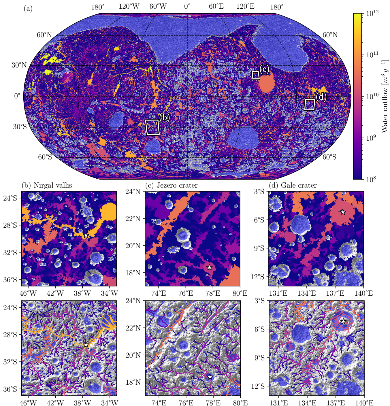
Figure 7. Water overflow at steady state with a GEL = 100 m. The color bar represents the water flow accumulation. The areas where there is no overflow are symbolized by white shaded areas and sky blue areas represent the watershed and lake/ocean areas. The first line of zoomed plots shows the raw output data of the hydrological model which represents the water overflow associated to the watershed area. The second line of zoomed plots shows the water overflow associated to the valley network, after post-processing explained in section 2.4.
