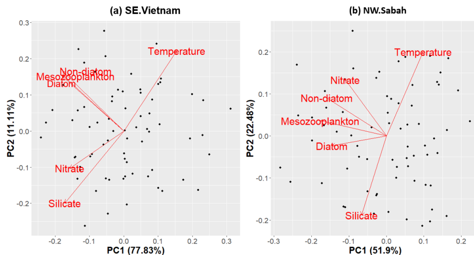
Figure 10: Principal Component Analysis (PCA) of seasonal means of phytoplankton biomass and the selected environmental variables in Southeast Vietnam(a) and Northwest Sabah(b) Regions (1990-2060). The arrows represent the variables, and the points represent the years. The arrows directed to same direction and are close to each other are positively correlated, arrows in opposite direction are negatively correlated and the arrows that are placed orthogonal have no relationship. It should be noted that vector orientation in PCA space reflects the contribution of each variable to the principal components, which capture directions of maximum shared variance across the full multivariate dataset. Apparent orthogonality between variables in the PCA biplot therefore reflects the absence of a shared variance structure along the principal component axes and does not necessarily contradict pairwise Pearson correlations computed independently between individual variables. Where discrepancies exist between PCA vector orientation and reported Pearson correlations, these should be interpreted with reference to the proportion of variance explained by each principal component and the potential influence of dominant variables on the ordination space.
