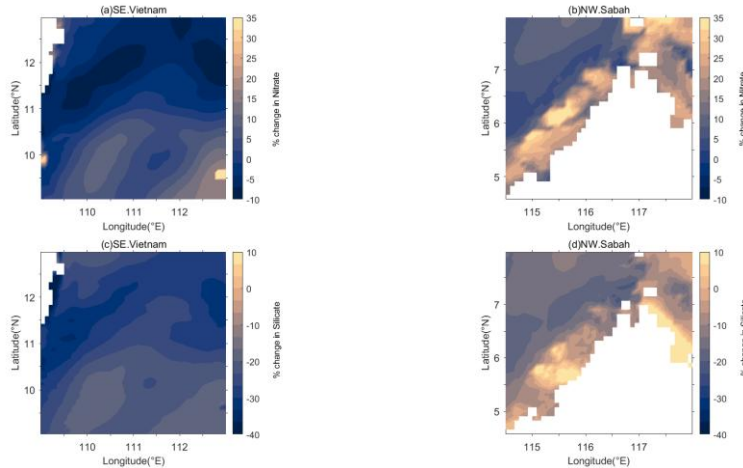
Figure 67: Percentage change in nitrate (a, b) and silicate (c, d) concentrations of the upper 120 m of the water column during the upwelling seasons in Southeast Vietnam (a, c) during summer and Northwest Sabah (b, d) during winter from 2050 to 2060 under the RCP8.5 scenario relative to the period 1990-2000.
