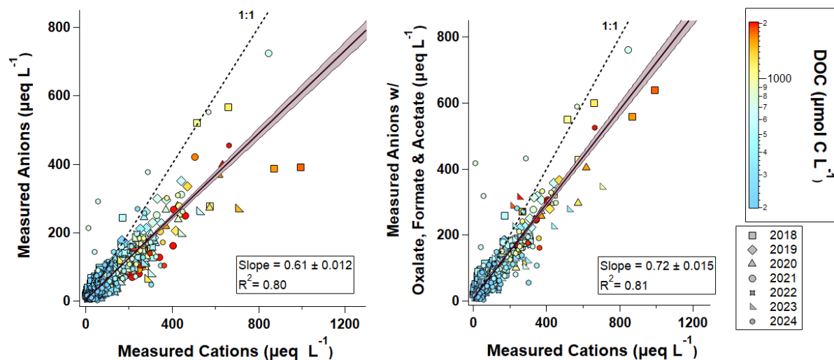
Figure S5. Measured anions versus cations in cloud water excluding and including the three major LMWOA in the left and right plots, respectively, colored by the measured DOC concentrations, with different marker shapes indicating different collection years. Slopes and linear correlation coefficients correspond to linear fits of all samples, with shaded area representing the 95% confidence band of the linear fit.
