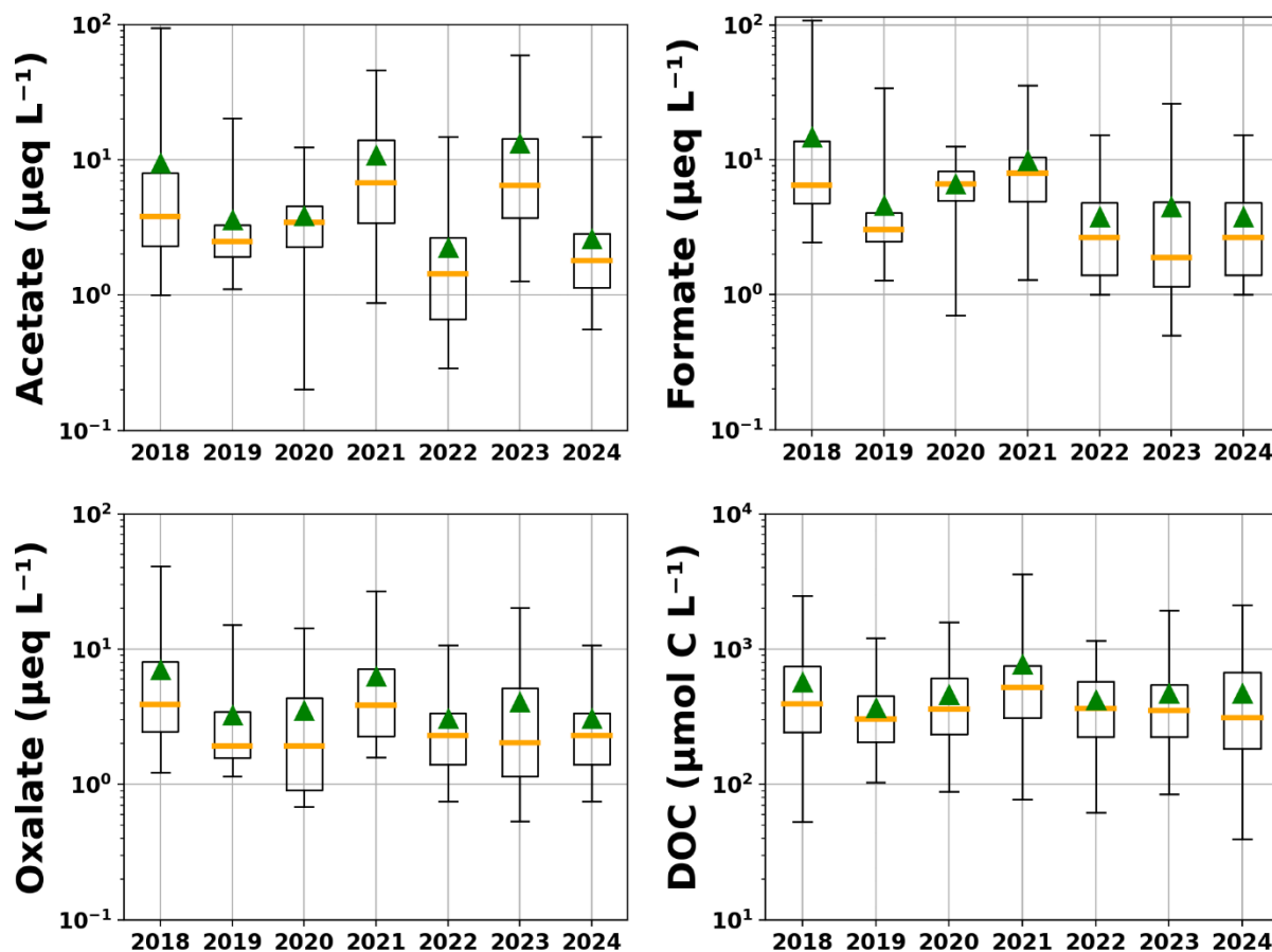
Figure S6. Box and whisker plots of yearly statistics for three LMWOA and DOC above detection limits in cloud water samples collected in summer. The orange line is the median concentration, and green triangle is the mean concentration. Whiskers extend from the 1 st to the 99 th percentiles.
