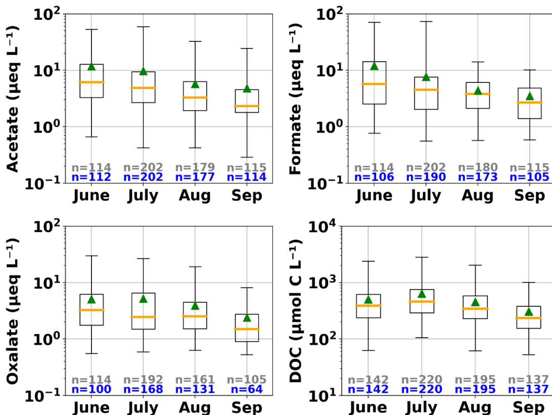
Figure S4. Box plots of monthly variation of 3 LMWOAs and DOC in cloud water at WFM during the collection season, n (in grey font) represents the number of total samples analyzed and n (in blue font) represents the number of samples reported in the plot above detection limit, orange line is the median and green triangle is the mean concentration, whisker extends from 1 to 99 percentile
