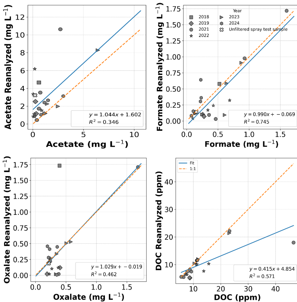
Figure S1. Linear regression plots of reanalyzed vs. original LMWOA (a) acetate, (b) formate, and (c) oxalate concentrations, and (d) DOC concentrations. Note that the linear fits on (a)-(c) do not include the unfiltered spray test sample, shown by the open “X” symbol.
