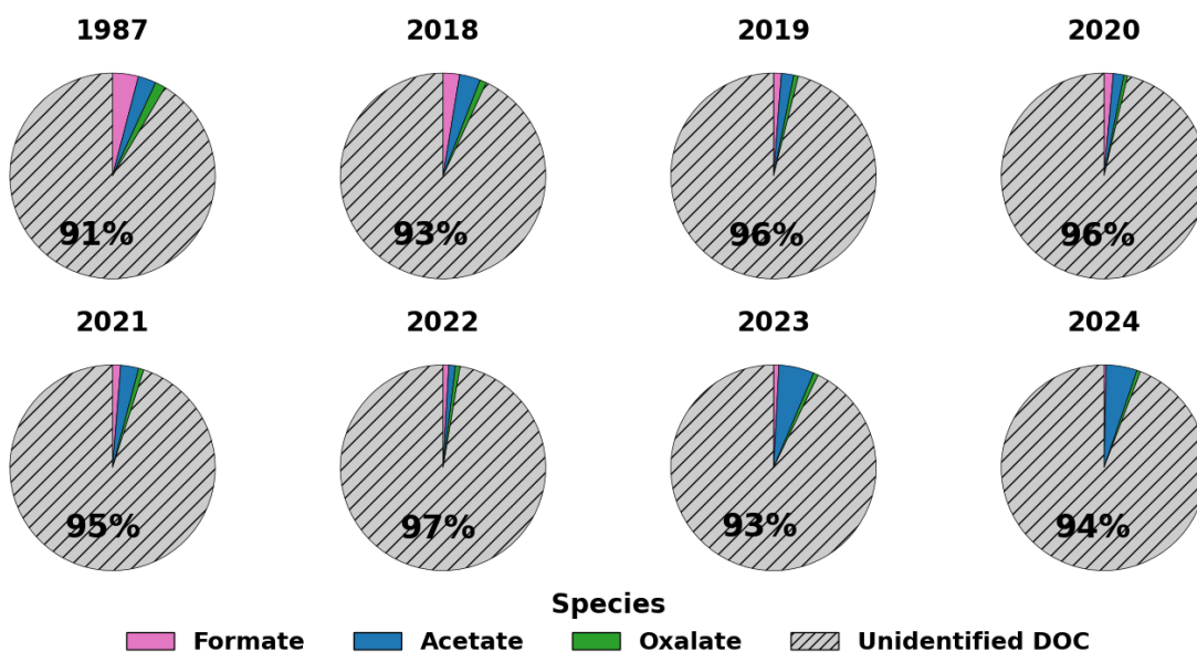
Figure S3. Annual mean contributions of measured low-molecular-weight organic acids to measured DOC concentrations in Whiteface Mountain cloud water (1987, 2018–2024)
