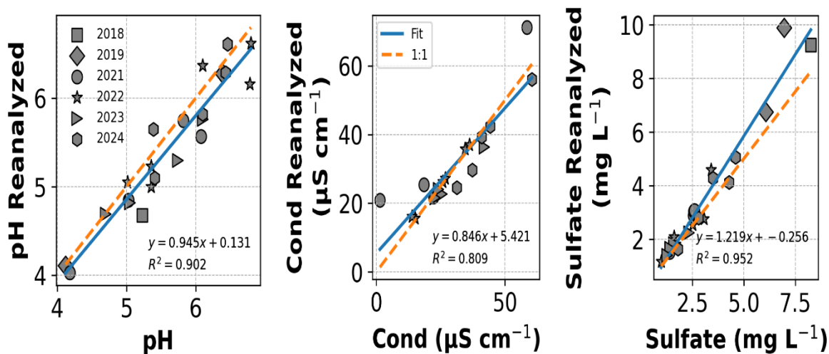
Figure S2. Linear regression plot of pH, conductivity and Sulfate (original vs reanalyzed concentrations)
