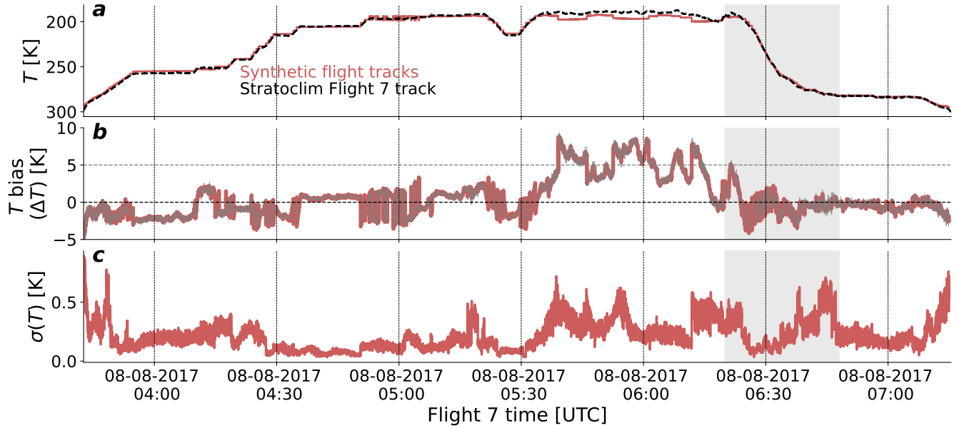
Figure 2. Temperature along the StratoClim Flight 7 track and the average temperature across the 20 synthetic flight tracks from the ICON IM00 simulation (panel a ). Temperature biases along the synthetic flight tracks relative to the in-situ measurements (panel b ). The temperature bias of the “best trajectory” for which bias is minimized most often is overlaid in gray. Standard deviation in temperature over the 20 synthetic flight tracks (panel c ). A period of continuous descent from 06:20–06:48 UTC is shaded in gray for all panels.
