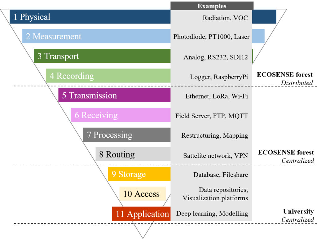
Figure 4: Layer model of the data collection.
