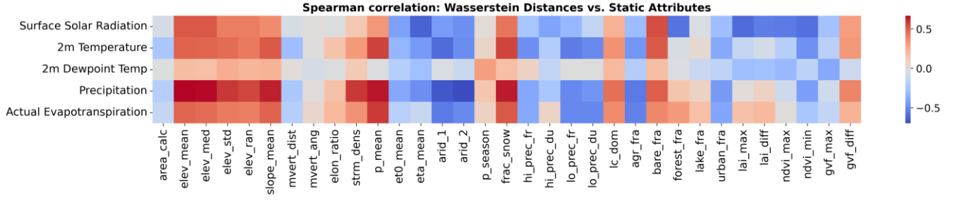
Figure 4. Spearman correlation between the per-basin 1-Wasserstein distances of five shared meteorological variables (Surface Solar Radiation, 2m Temperature, 2m Dewpoint Temperature, Precipitation, Actual Evapotranspiration) and 33 static catchment attributes across all 451 basins during the test period (2014–2017). Positive values (red) indicate that catchments with larger values of a given attribute tend to experience larger distributional differences between ERA5-Land reanalysis and ECMWF-HRES forecast inputs, while negative values (blue) indicate smaller distributional differences. Wasserstein distances are computed in the original physical units of each variable using the domains from the cross-domain evaluation experiment.
