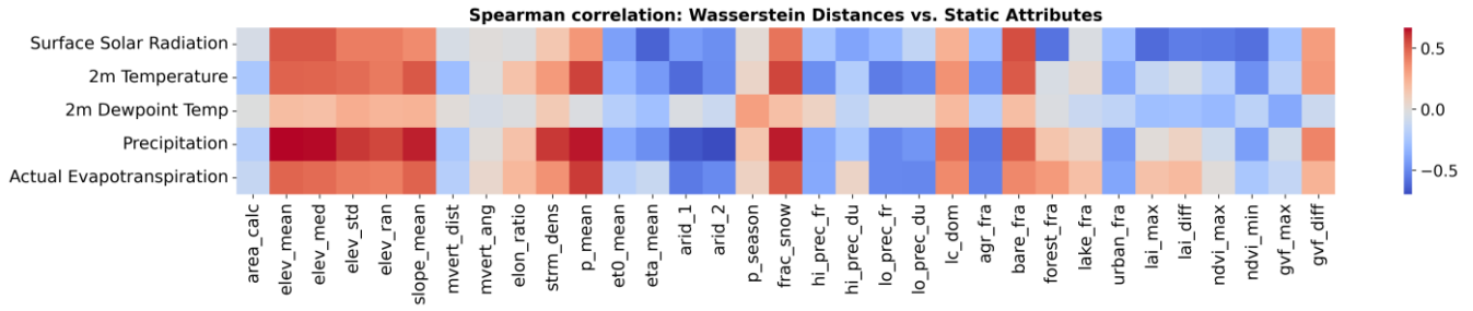
375 Figure 4. Spearman correlation between the per-basin 1-Wasserstein distances of five shared meteorological variables (Surface Solar Radiation, 2m Temperature, 2m Dewpoint Temperature, Precipitation, Actual Evapotranspiration) and 33 static catchment attributes across all 451 basins during the test period (2014–2017). Positive values (red) indicate that catchments with larger values of a given attribute tend to experience larger distributional differences between ERA5-Land reanalysis and ECMWF-HRES forecast inputs, while negative values (blue) indicate smaller distributional differences. Wasserstein distances are computed in the original physical units of each variable using the domains from the cross-domain evaluation experiment.
