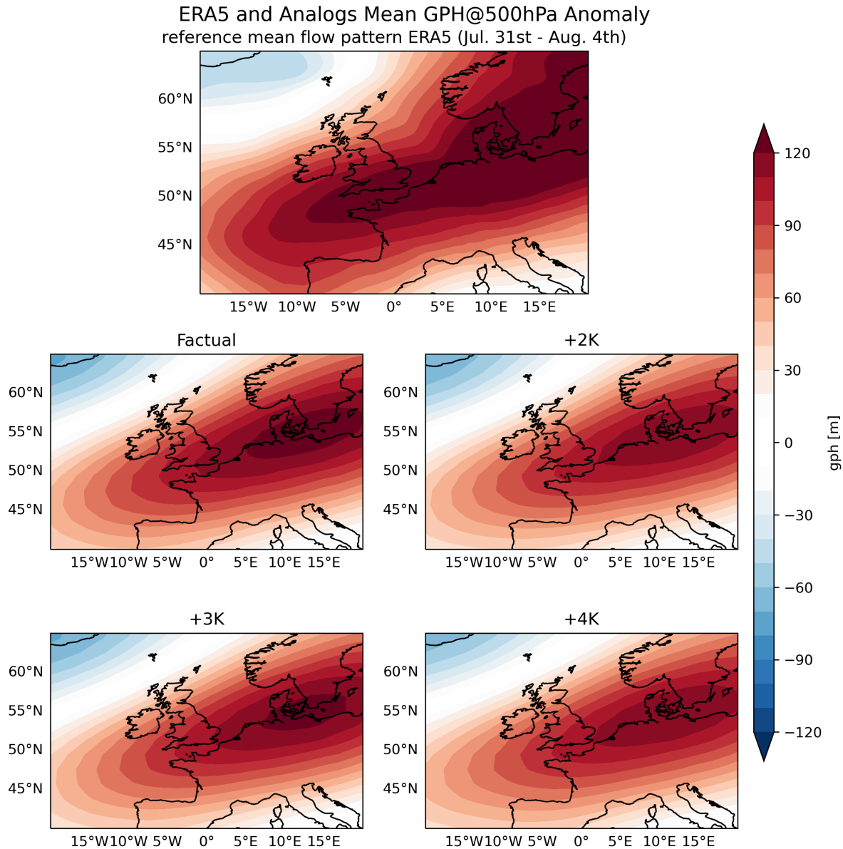
Figure S4. ERA5 and analogues' ensemble mean time-averaged GPH@500hPa anomaly. The fields portrayed for Factual, +2K, +3K, and +4K correspond to the 5-day time-average from the N analogues detected out of the 50 members in the MPI-ESM-LR Grand Ensemble.
