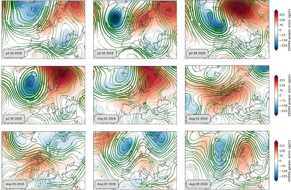
Figure S6. Geopotential height anomaly and wind velocity at 500hPa during the entire heatwave event (July 24th - August 10th). The sequence shows every 2-day flow patterns, with wind streamlines showing wind velocity. The anomalies are relative to the 1985-2014 climatology mean.
