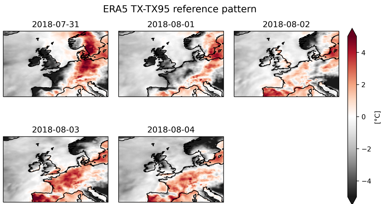
Figure S2. ERA5 Reference temperature anomaly. 5-day sequence of daily maximum temperature anomaly relative to the 95th percentile of the 1985-2014 climatology.
