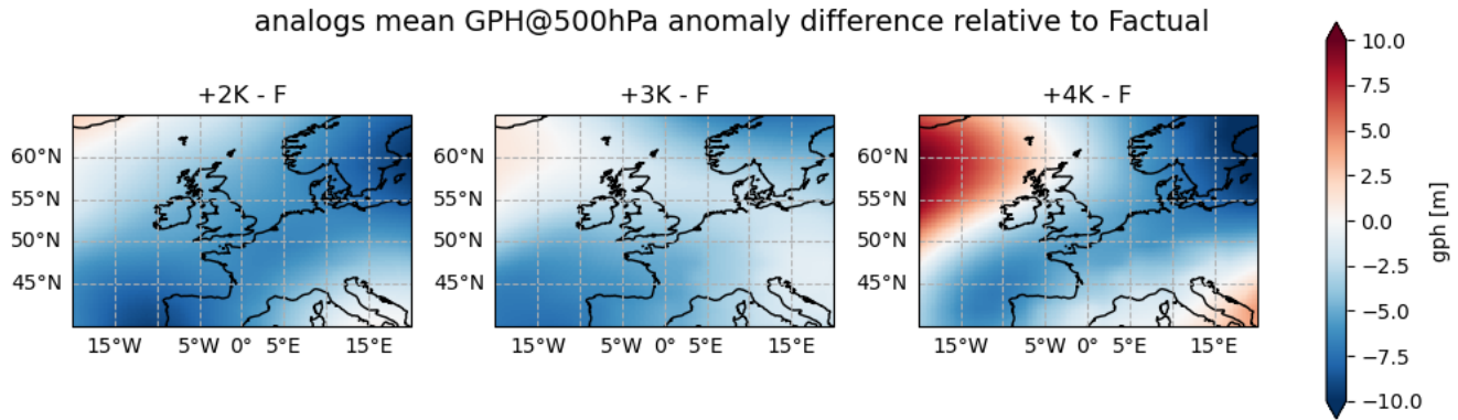
Figure S5. Analogues mean GPH@500hPa anomaly difference for future levels of global warming relative to factual (present times). Differences include the ensemble mean of the 5-day sequence for each analogue detected at each level of global warming.
