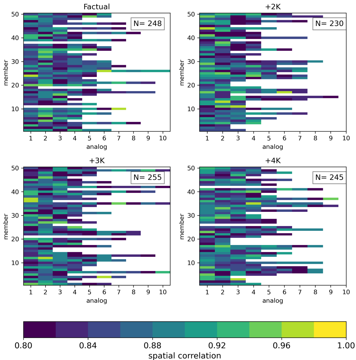
Figure S3. Flow-analogue's spatial correlation matrix relative to ERA5 reference flow pattern per degree of global warming level. Each correlation matrix shows the spatial correlation of analogues detected for each ensemble member of the MPI-ESM-LR Grand Ensemble. The label N corresponds to the total number of analogues identified in such a dataset.
