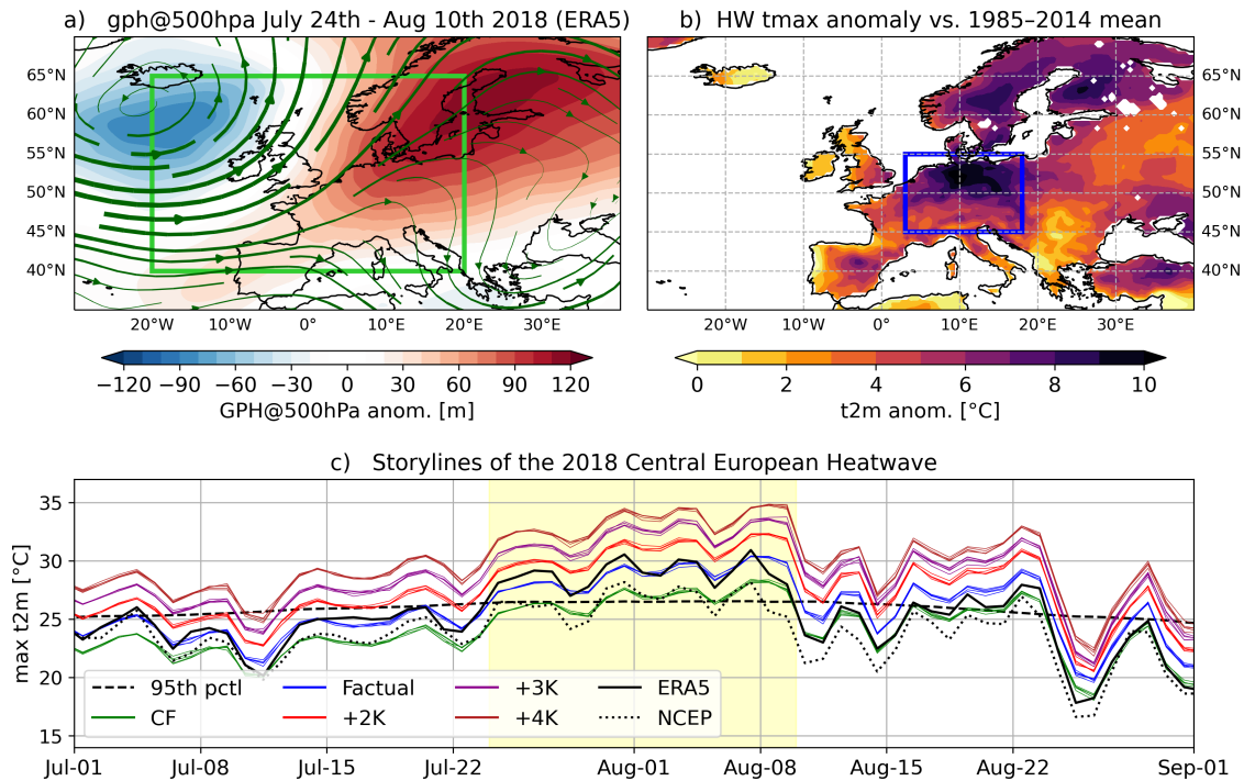
Figure 2. Heatwave intensity–The 2018 Central European heatwave. a–e) Local maximum heatwave intensity–Mean geopotential height anomaly (gph@500hPa) and streamlines based on 500 hPa mean wind components during the heatwave event of interest (July 24th–August 10th). The green box encloses the region (20° W, 20° E, 40° N, 65° N) used for each storyline flow-analogue detection. fb) Time-series of daily Maximum near-surface temperature anomaly with respect to mean climatology during the heatwave intensity-over event. The blue box encloses the region of interest (Central Europe: 3° E, 18° E, 44° N, 55° N) enclosed in blue boxes. The stars in the c) Daily maximum temperature time series plot are the heatwave mean intensity per spatially averaged over Central Europe for each storyline (magnitudes shown in CF: counterfactual, factual, +2K, +3K, +4K), counting on 5 members each (thin lines). The dashed line corresponds to the upper left corner 95th percentile of the maps 1985–2014 climatology. The black solid line corresponds to ERA5 data for comparison to the factual world. The yellow shaded region encloses the length of the event in the factual world (July 24th–August 10th).
