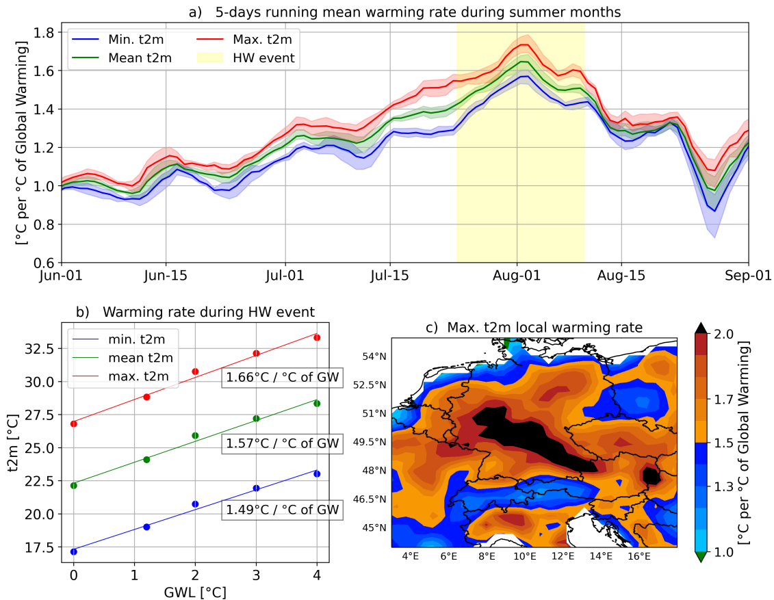
Figure 4. Warming rate: 2 meter temperature increase per degree of global warming. Warming rate: 2 meter temperature increase per degree of global warming. a) 5-day running average warming rate for minimum (blue), mean (green), and maximum (red) near-surface temperature spatially averaged over Central Europe. Color shading corresponds to the range covered by the 5 available members. b) Mean warming rate during the July 2018 heatwave event per degree of global warming ( counterfactual, factual, +2K, +3K, +4K ) spatially-averaged over Central Europe. c) Local warming rate of the event's mean maximum temperature over the region of interest (Central Europe).
