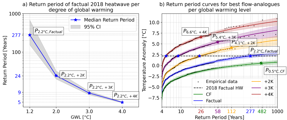
Figure 7. Heatwave intensity's return periods. a) Return period of the factual 2018 HW per degree of global warming. b) Return periods of heatwave intensity for each global warming level (counterfactual, factual, +2K, +3K, +4K). Solid lines show return levels obtained through GEV fitting of 250 analogue events scaled by their 1-in-4 years occurrence out of the 1000 years sampled (50 members x 20 years). Shaded regions enclose the 95% confidence interval (lower bound: 2.5th percentile, upper bound: 97.5th percentile) obtained by a 1000-sample bootstrap resampling. Stars show the return period equivalent to the projected intensity by the storyline approach.
