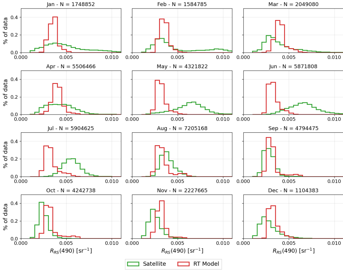
Figure 8. Monthly distributions of sea surface reflectance at 490 nm in 2018 across the Black Sea basin, from the RT configuration (in red) and remote-sensing (in green) . Simulated reflectance is interpolated at the location of available remote-sensing data.
