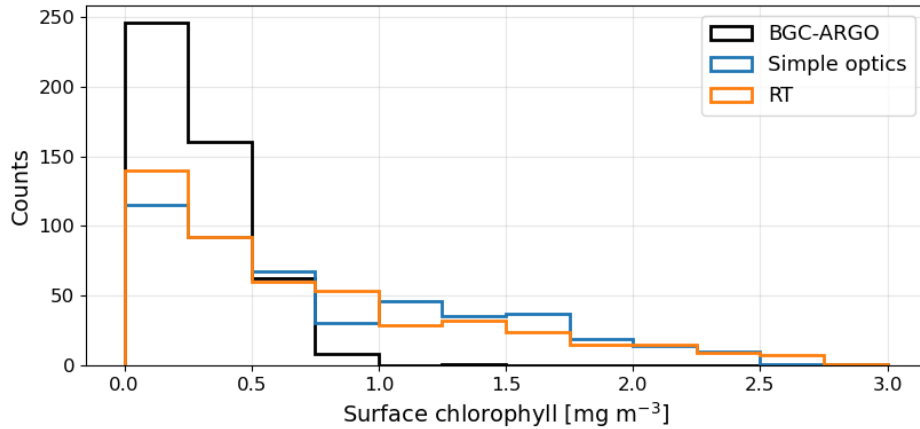
Figure 7. Distributions of surface chlorophyll compared with data from BGC-Argo floats (in black) between 2017 and 2020. Distributions of matching surface chlorophyll from the simple optics and RT configurations are respectively shown in blue and orange. 478 profiles are represented here for the simple optics and RT configurations. Bin width is here set to 0.25 mg m -3
