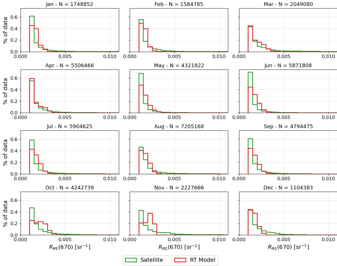
Figure 10. Monthly distributions of sea surface reflectance at 670 nm in 2018 across the Black Sea basin, from the RT configuration (in red) and remote-sensing (in green) . Simulated reflectance is interpolated at the location of available remote-sensing data.
