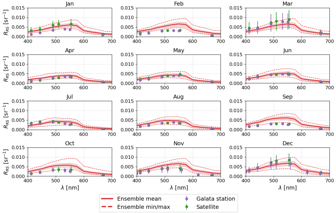
Figure 14. Monthly composites of sea surface reflectance spectra in 2018 at the Galata station (43.045°N, 28.193°E, Romania ). Remote-sensing data are taken at the closest grid point to the Galata station. For observations, points represent the average R_{RS} for the month and bars represent one standard deviation in the data of the month. Model results are taken from the stochastic RT configuration with the ensemble mean in bold lines, the ensemble standard deviation in shaded, and the ensemble minimum and maximum in dotted lines.
