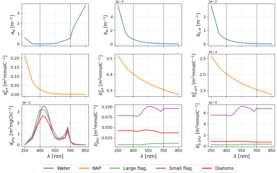
Figure 1. Optical Spectra for the optical properties for water (top) (Pope and Fry, 1997), non-algal particles (centre) (Gallegos et al., 2011; Álvarez et al., 2022) and the three PFTs defined in BAMHBI: diatoms, small flagellates and large flagellates (bottom) (adapted from Dutkiewicz et al., 2015; Álvarez et al., 2022).
