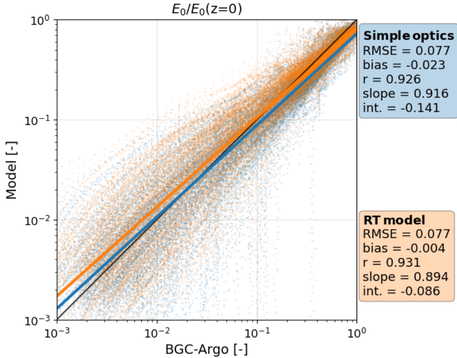
Figure 5. Logarithm of normalised \text{PAR-}E_0 derived from BGC-Argo data with the simple optics and RT configurations at the location of BGC-Argo floats between 2017 and 2020, for the upper 100 metres. RMSE, bias correlation coefficient ( r ), regression slope and intercept are displayed. Scatter plots show 36 376 data points. Normalisation is performed relative to the maximum value of the \text{PAR-}E_0 profile, which is the closest data from sea surface.
