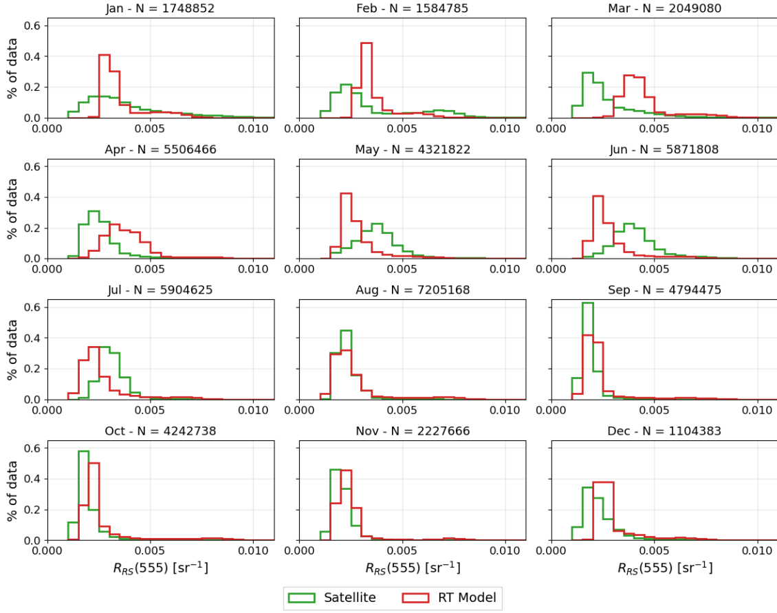
Figure 9. Monthly distributions of sea surface reflectance at 555 nm in 2018 across the Black Sea basin, from the RT configuration (in red) and remote-sensing (in green) . Simulated reflectance is interpolated at the location of available remote-sensing data.
