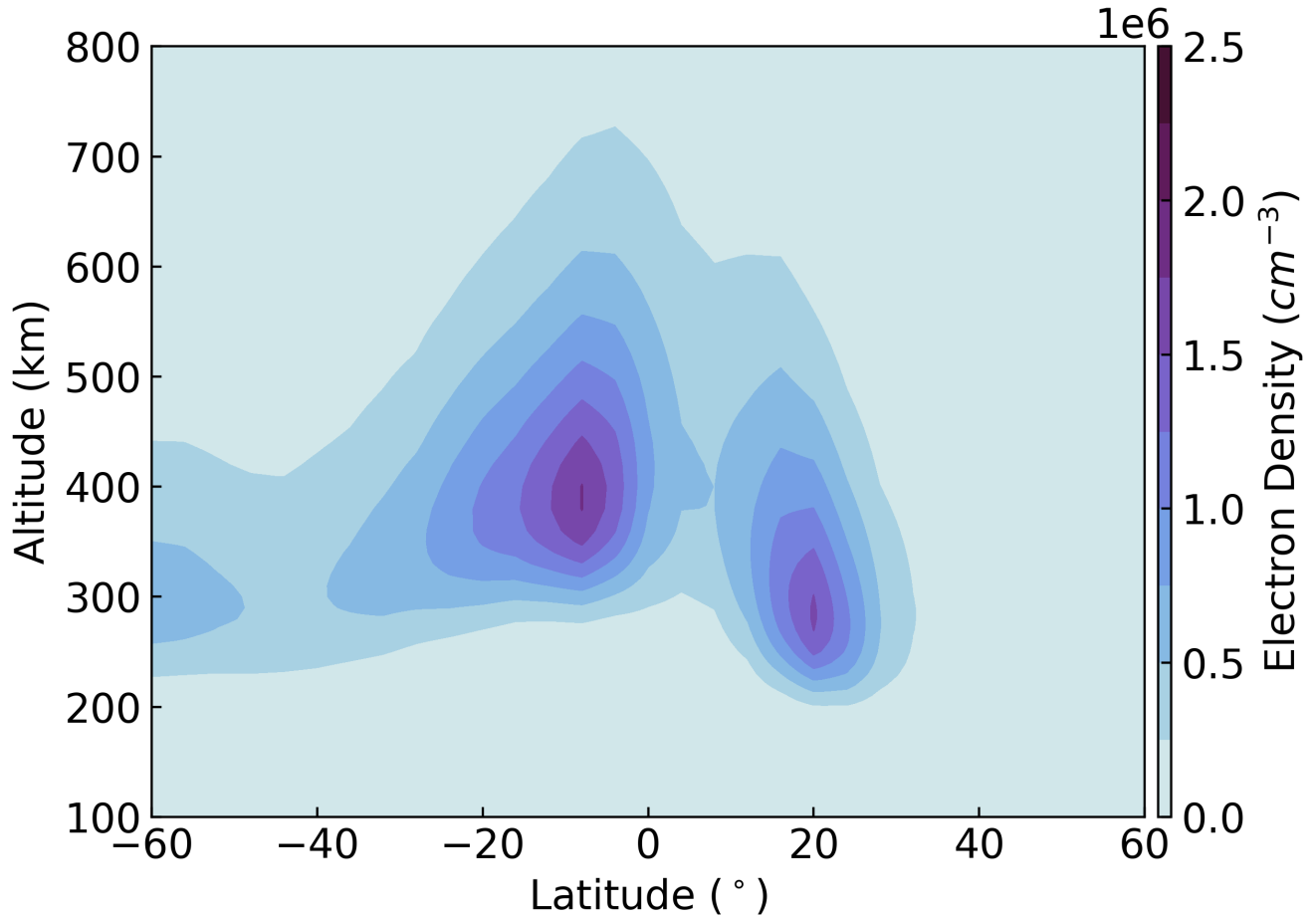
Figure 2. NIMO specification of electron density as a function of latitude and altitude at a longitude of 90°E at 15:00 UT for 19 Jan 2014.
