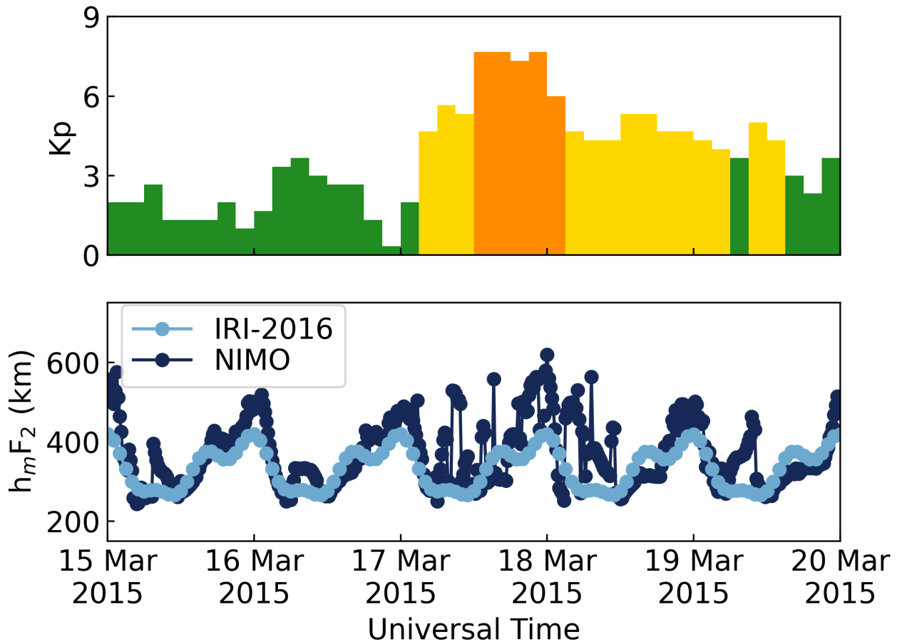
Figure 10. Kp (top panel) and h_m F_2 (bottom panel) for the Mar 2015 storm period.
