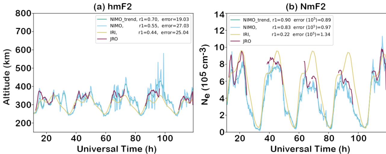
Figure 11. h_mF_2 (a) and N_mF_2 (b) for the JRO ISR starting at 6 Jan 2021 11:20 UT. The ISR observations are shown by purple lines, the NIMO results are plotted in blue, the NIMO trend is plotted in green, and the IRI-2016 results are plotted in yellow. Note how the purple JRO h_mF_2 generally lies in the middle of the NIMO h_mF_2 and shows similar local time variations to the NIMO N_mF_2 , while the IRI-2016 values consistently have local time variations not consistent with the observations.
