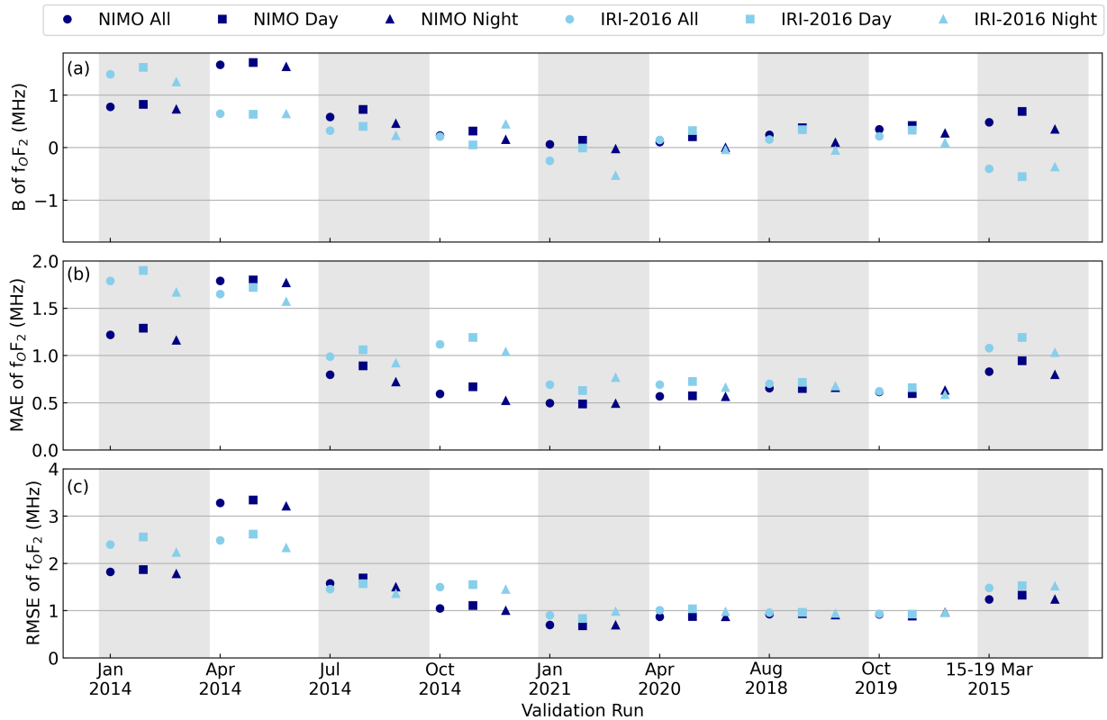
Figure 8. Global f_oF_2 B (a), MAE (b), and RMSE (c) in different local time bins for all ionosonde locations.
