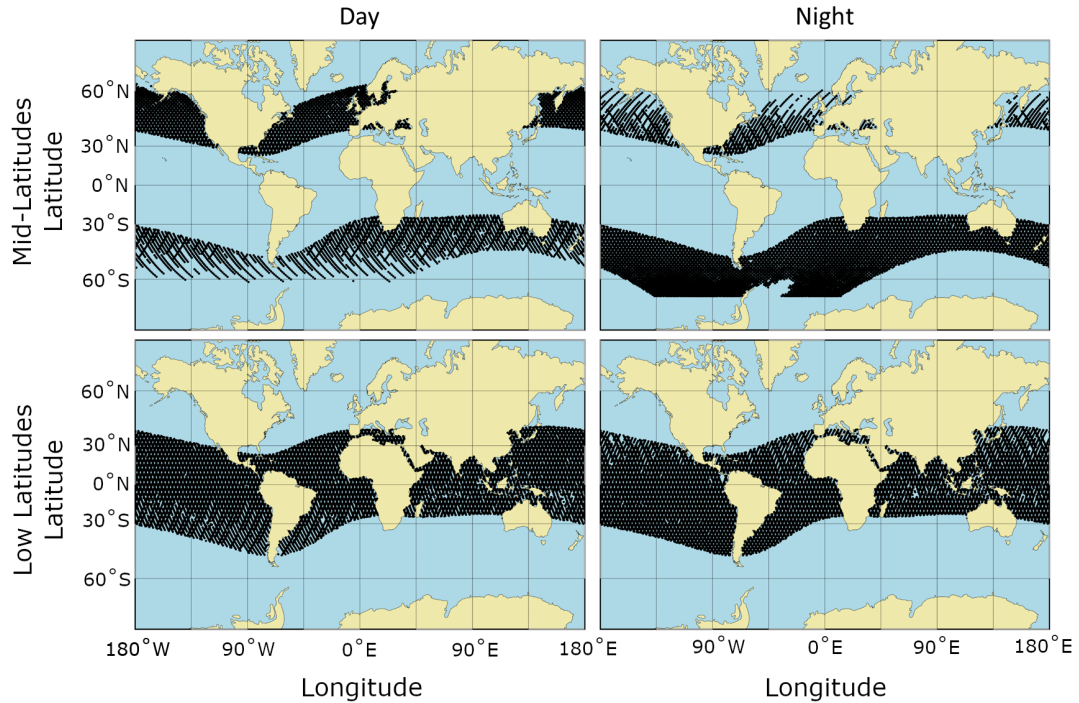
Figure 16. JASON-2 data coverage in Jan 2014 as a function of latitude and longitude for the mid- and low-latitudes at daytime and nighttime. For this report, we define mid-latitudes as latitudes between 60^\circ and 35^\circ north and south of the magnetic equator. Low-latitudes include regions within 35^\circ of the magnetic equator. Daytime passes include local times between 06:00 SLT and 18:00 SLT, and nighttime passes are between 18:00 SLT and 06:00 SLT.
