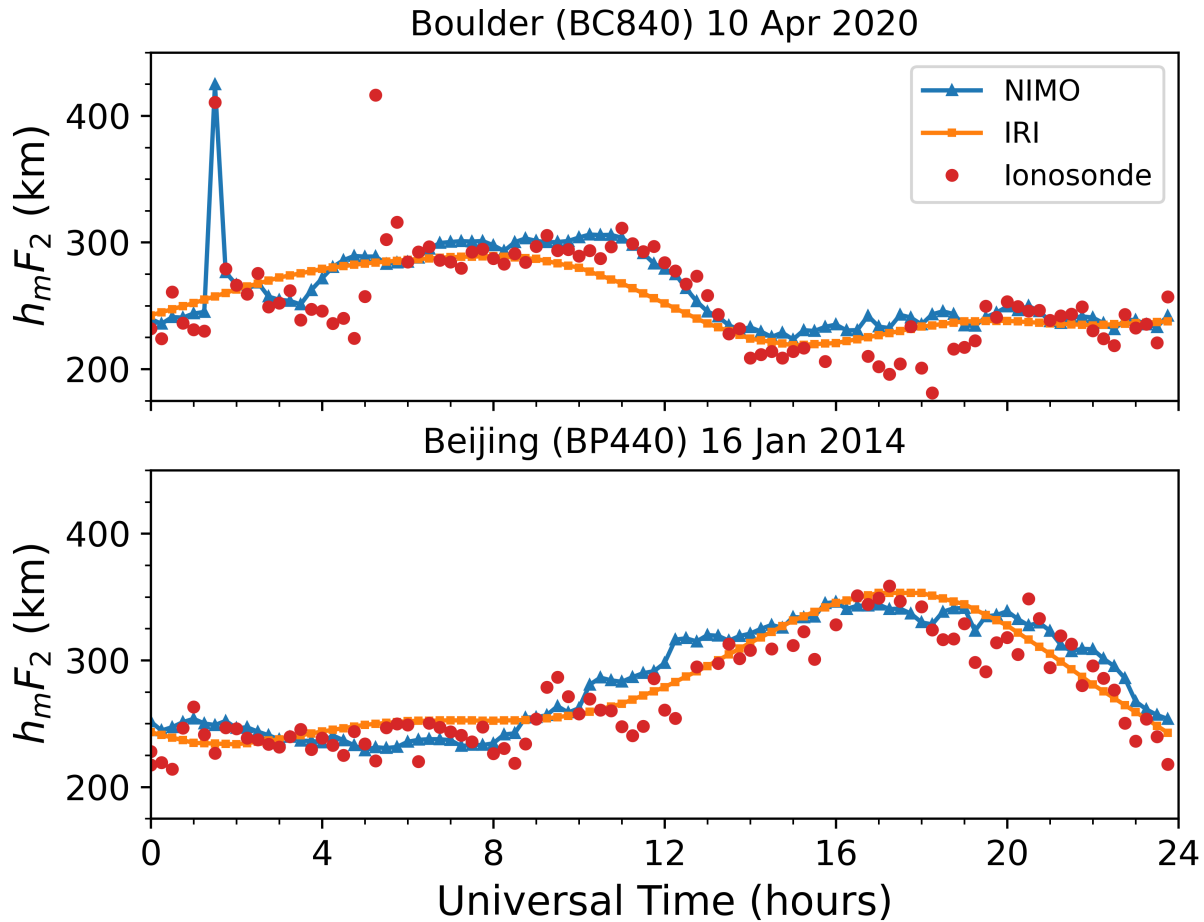
Figure 7. h_mF_2 for ionosonde station locations at Boulder, USA (top) and Beijing, China (bottom). The ionosonde observations are shown by red dots, while the NIMO results are plotted in blue lines and triangles and the IRI-2016 results are plotted in orange lines and squares.
