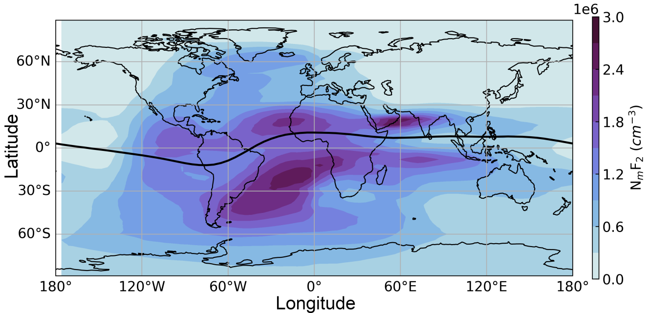
Figure 3. NIMO specification of global peak electron density in the F region at 15:00 UT for 19 Jan 2014.
