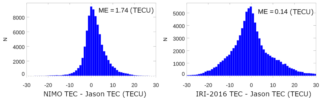
Figure 20. Difference histograms of the TEC between the models NIMO (left) and IRI-2016 (right) and JASON-2 in Jan 2014.
