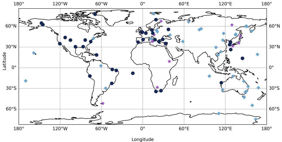
Figure 4. Map of ionosonde locations used for data assimilation and validation. The purple stars are sites that are only used for data assimilation. The light blue diamonds are sites that are used for validation only. The navy circles are sites that are used for ingestion and validation.
