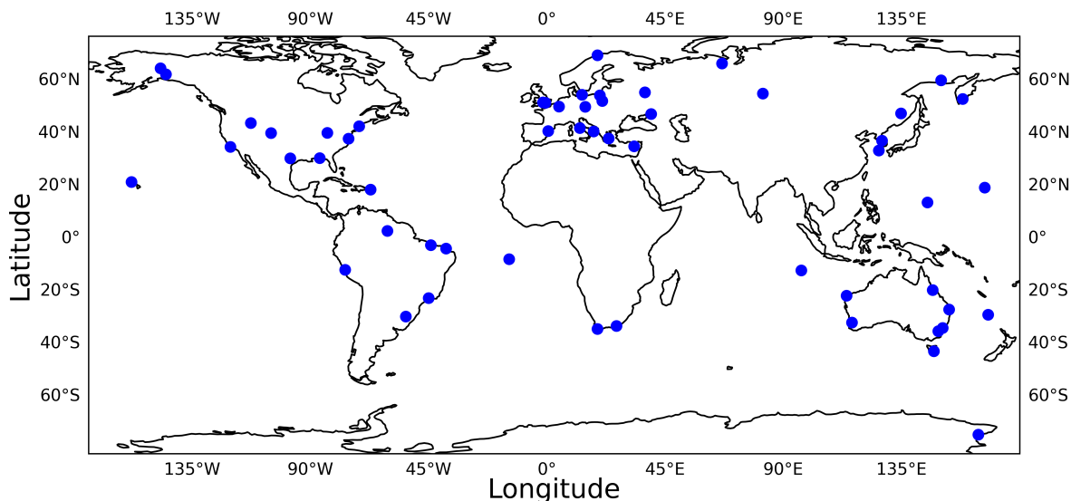
Figure 4. Map of ionosonde locations used for validation.
