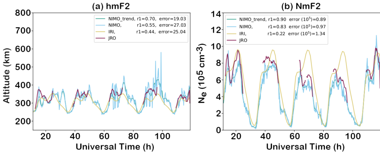
Figure 11. h_mF_2 (a) and N_mF_2 (b) for the JRO ISR starting at 6 Jan 2021 00:00 UT. The ISR observations are shown by purple lines, the NIMO results are plotted in blue, the NIMO trend is plotted in green, and the IRI-2016 results are plotted in yellow. Note how the purple JRO h_mF_2 generally lies in the middle of the NIMO h_mF_2 and shows similar local time variations to the NIMO N_mF_2 , while the IRI-2016 values consistently have local time variations not consistent with the observations.
