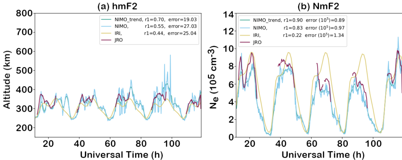
Figure 11. h_mF_2 (a) and N_mF_2 (b) for the JRO ISR starting at 6 Jan 2021 0011:00-20 UT. The ISR observations are shown by purple lines, the NIMO results are plotted in blue, the NIMO trend is plotted in green, and the IRI-2016 results are plotted in yellow. Note how the purple JRO h_mF_2 generally lies in the middle of the NIMO h_mF_2 and shows similar local time variations to the NIMO N_mF_2 , while the IRI-2016 values consistently have local time variations not consistent with the observations.
