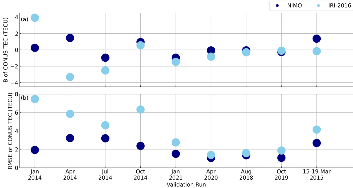
Figure 14. CONUS TEC B (a) and RMSE (b) for all validation runs.
