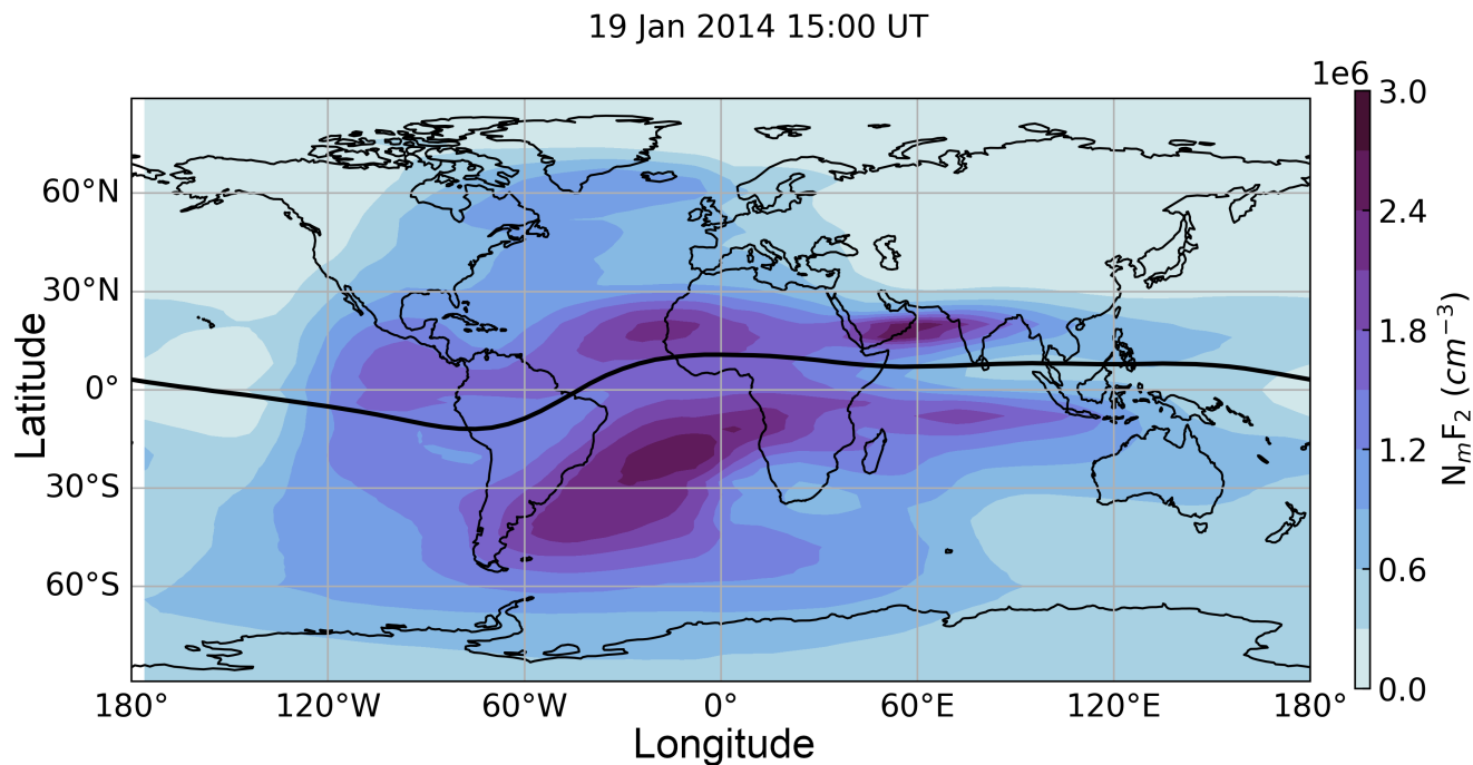
Figure 3. NIMO specification of global peak electron density in the F region at 15:00 UT for 19 Jan 2014.
