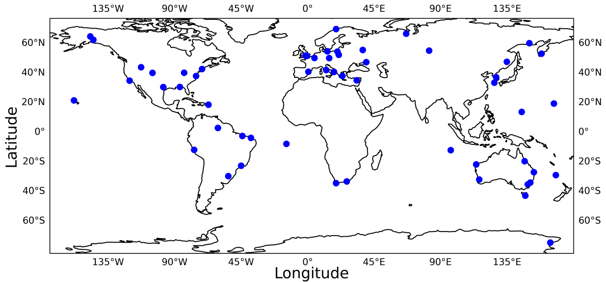
Figure 4. Map of ionosonde locations used for validation.
