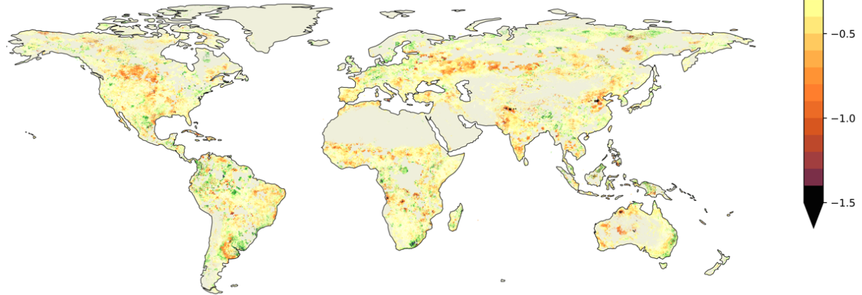
Figure 7. Spatial pattern of the mean GPP SA during MYDs for a) MODIS and b) LPJmL-5. Positive values indicate higher GPP than normal during MYDs, while negative values indicate reduced GPP values. Bare areas and sparse vegetation are filtered out. c) shows a violin plot comparing the distributions of the mean GPP SA during MYDs from MODIS and LPJmL-5.
