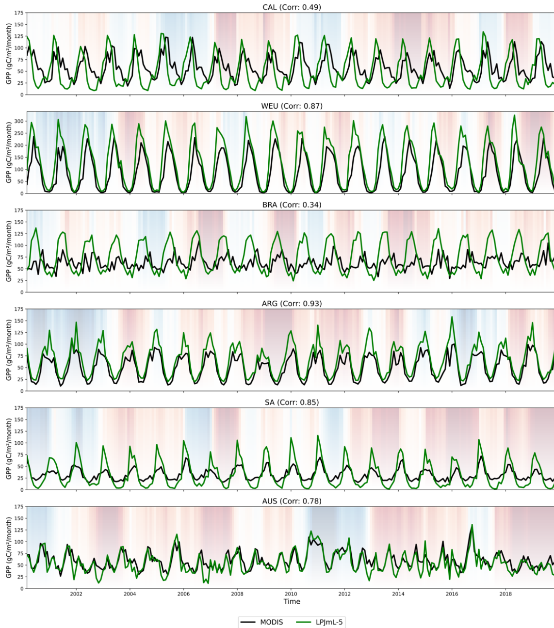
Figure 4. Timeseries – Time series of the GPP for LPJmL-5 with prescribed land cover (green) and MODIS (black) for the focus regions: California (CAL), western Europe (WEU), Brahmaputra (BRA), middle Argentina (ARG), southern Africa (SA) and the Murray Darling Basin in Australia (AUS). SPEI-12 is shaded in the background, where red areas indicate drier periods and blue areas wetter periods. Additionally, the figure includes the correlation between MODIS and LPJmL-5 per region. Note that WEU uses a different y-axis range from the other regions.
