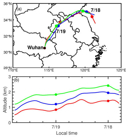
Figure 3. HYSPLIT three two-day backward trajectories starting from Wuhan (30.5° N, 114.4° E) at 1900 LT on 19 July 2019 at altitudes of 0.5, 0.8, and 1.2 km. The solid dots represent 00 LT for each day.
