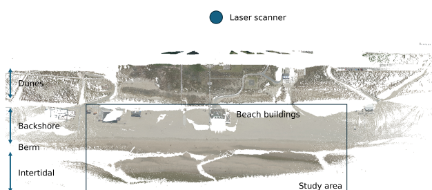
Figure 3. Permanent laser scanning point cloud of the study area indicating the main morphological beach units and cross-shore area featuring buildings. The scan is coloured using aerial photos of the Dutch government (pdok/beeldmateriaal.nl)
