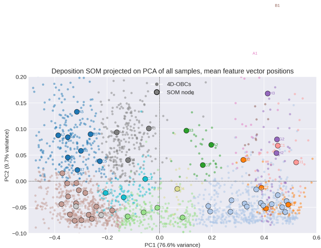
Figure A1. Space defined by the first two principal components of the features of the deposition 4D-OBCs. Small dots indicate transformed 4D-OBC positions in PCA space, larger dots indicate the transformed location of the mean feature vectors of the Self-organizing Map (SOM). The colours relate to the colours in Fig. 8.
