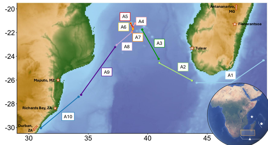
Figure 1. Location of the 10 aerosol samples, numbered A1 to A10, collected during the RESILIENCE cruise in the Southern Mozambique Channel. The inset world map indicates the location of this study (yellow rectangle) together with the location of previous field studies (symbols) reporting atmospheric trace element concentrations in the direct vicinity of our study region (triangle: Witt et al. (2006), circle: Witt et al. (2010), star: Chester et al. (1991)).
