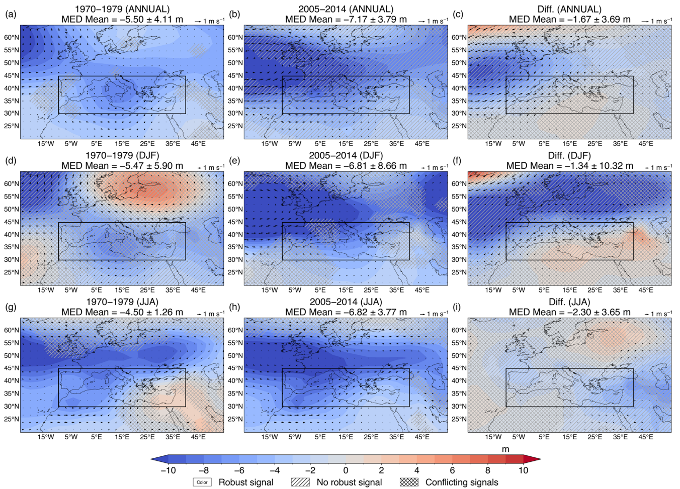
800 Figure 10. Changes in geopotential height and winds at 850 hPa due to anthropogenic aerosols over the Mediterranean (calculated from the difference historical minus hist-piAer ). Spatial patterns are presented for the periods 1970–1979 (left column), 2005–2014 (middle column) and their difference (2005–2014 minus 1970–1979; right column) on an annual scale (top row) and in boreal winter (DJF; middle row) and summer (JJA; bottom row). The multi-model ensemble means over the Mediterranean region (shown as a box) are shown along with the inter-model variability (one standard deviation) at the top of each panel. Colored areas without markings indicate robust changes, while hatched (/) and cross-hatched (X) areas indicate non-robust changes and conflicting signals, respectively.
