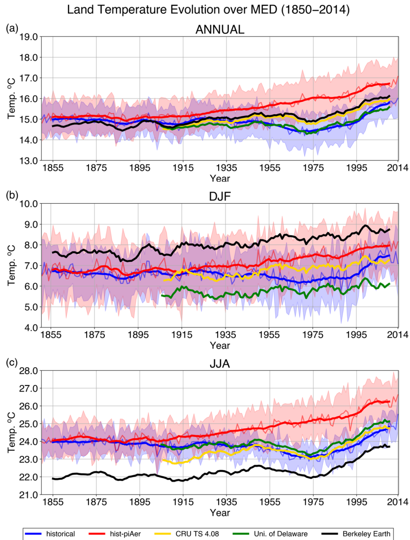
Figure 6. Timeseries of land TAS evolution over the Mediterranean region ( 10^{\circ}\text{W} – 40^{\circ}\text{E} , 30^{\circ}\text{N} – 45^{\circ}\text{N} ) for the historical period (1850–2014) as captured by CMIP6 ESMs and observations on an annual scale (top row) and in boreal winter (DJF; middle row) and summer (JJA; bottom row). Thick lines represent 10-year moving averages. In the cases of the CMIP6 experiments, the thin lines represent the annual weighted mean values, and shading indicates the inter-model variability expressed as one standard deviation.
