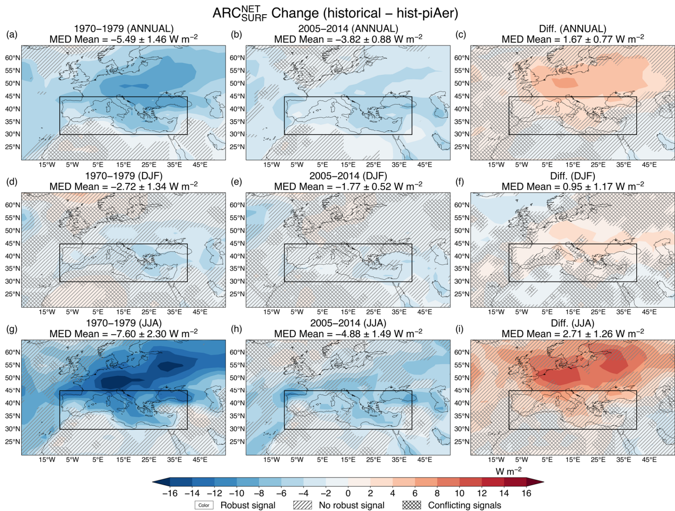
Figure 4. Net ARC SURF due to anthropogenic aerosols over the Mediterranean (calculated from the difference historical minus hist-piAer ).
