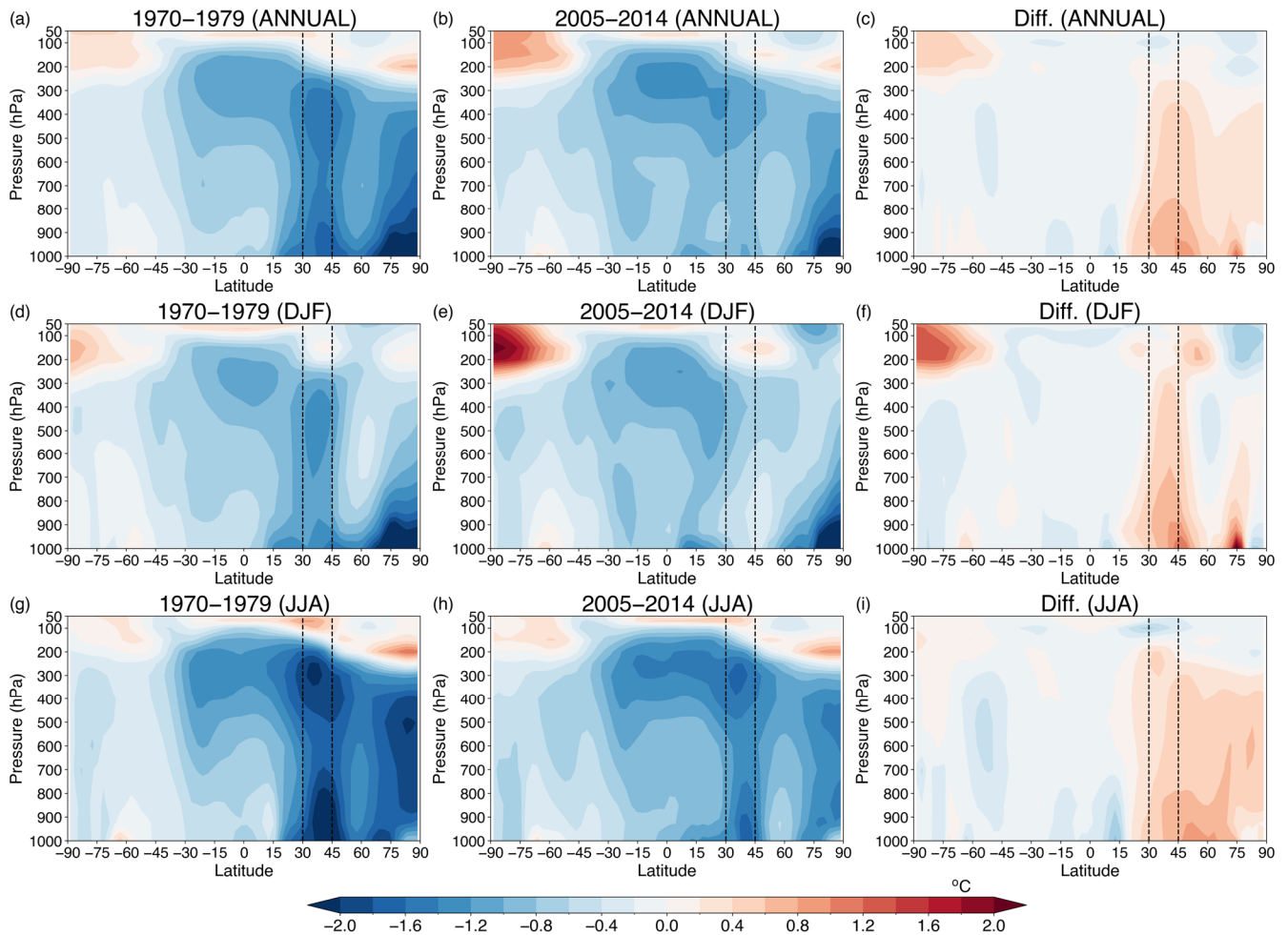
Figure 8. Changes in zonal mean temperature due to AAs (calculated from the difference historical minus hist-piAer ) for the MED longitudes (10°W – 40°E). Cross sections (pressure level over latitude) are presented for the periods 1970–1979 (left column), 2005–2014 (middle column) and their difference (2005–2014 minus 1970–1979; right column) on an annual scale (top row) and in boreal winter (DJF; middle row) and summer (JJA; bottom row). Dashed vertical lines indicate the latitudinal boundaries of the MED region.
