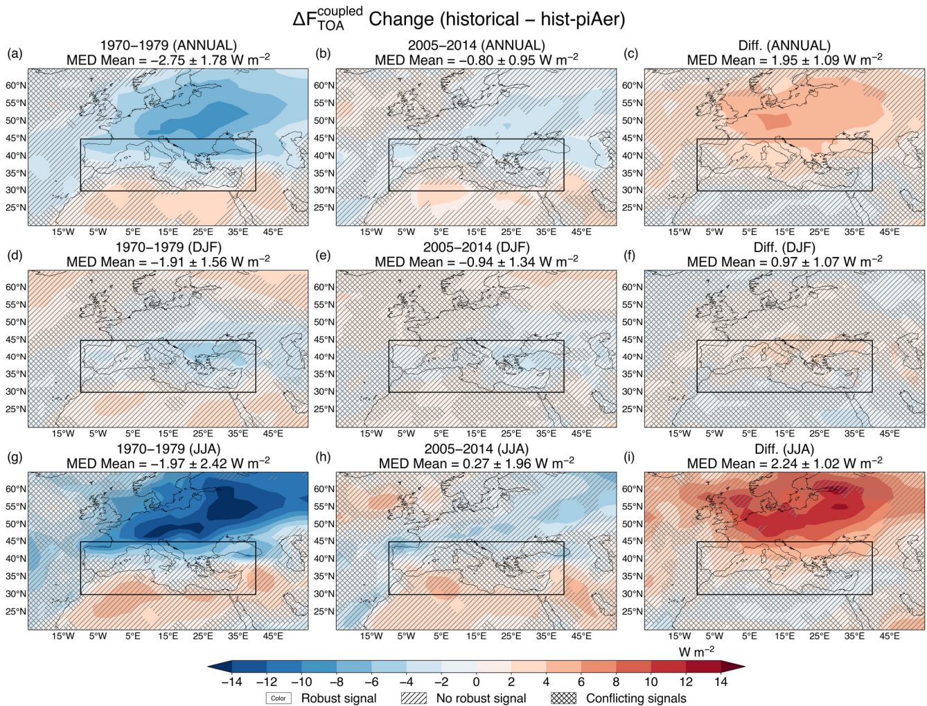
Figure 4. \Delta F_{\text{coupled}} at TOA due to anthropogenic aerosols over the Mediterranean (calculated from the difference historical minus hist-piAer ).
