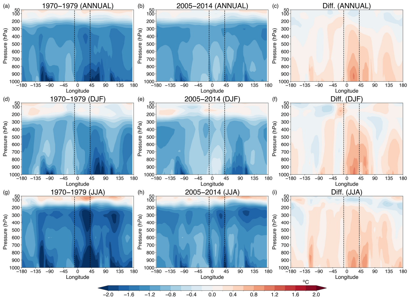
775 Figure 9. Changes in meridional mean temperature due to AAs (calculated from the difference historical minus hist-piAer ) for the MED 780 latitudes (30°N – 45°N). Cross sections (pressure level over longitude) are presented for the periods 1970–1979 (left column), 2005–2014 (middle column) and their difference (2005–2014 minus 1970–1979; right column) on an annual scale (top row) and in boreal winter (DJF; 785 middle row) and summer (JJA; bottom row). Dashed vertical lines indicate the longitudinal boundaries of the MED region.
