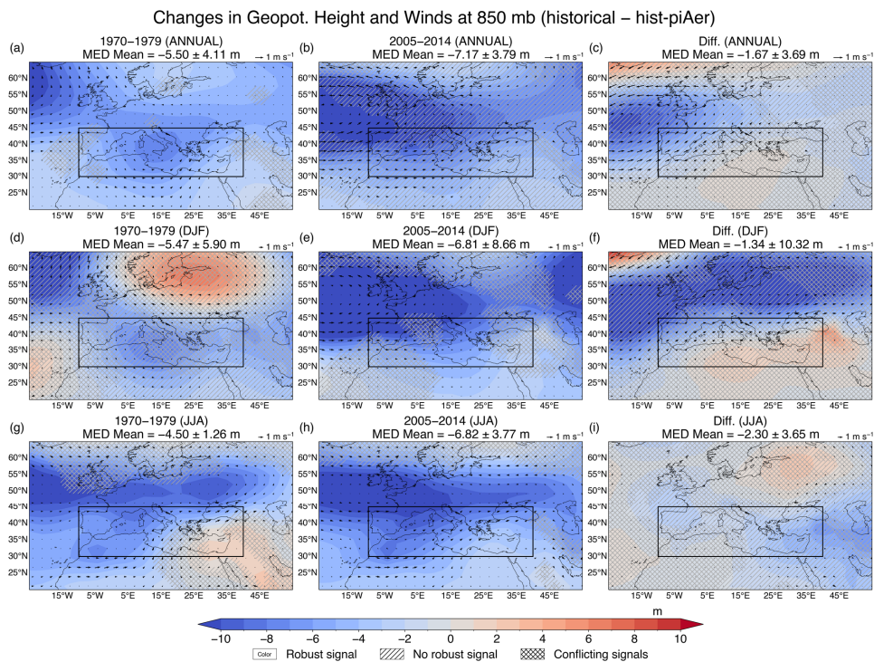
860 Figure 10. Changes in geopotential height and winds at 850 hPa due to anthropogenic aerosols over the Mediterranean (calculated from the difference historical minus hist-piAer ). Spatial patterns are presented for the periods 1970–1979 (left column), 2005–2014 (middle column) and their difference (2005–2014 minus 1970–1979; right column) on an annual scale (top row) and in boreal winter (DJF; middle row) and summer (JJA; bottom row). The multi-model ensemble means over the Mediterranean region (shown as a box) are shown along with the inter-model variability (one standard deviation) at the top of each panel. Colored areas without markings indicate robust changes, while hatched (/) and cross-hatched (X) areas indicate non-robust changes and conflicting signals, respectively. 865
