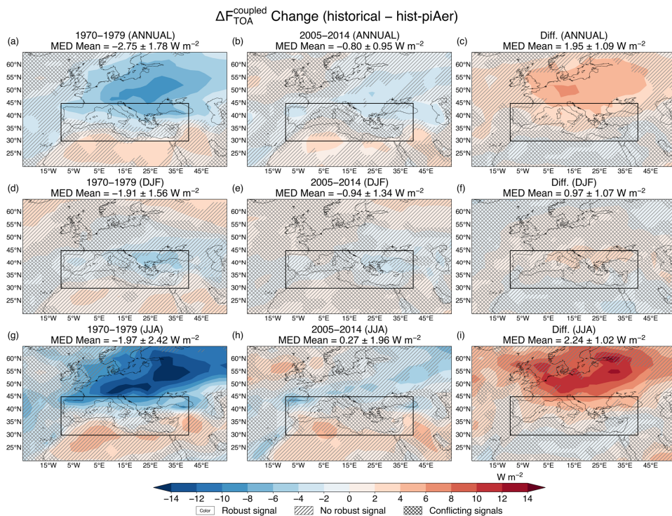
Figure 4. Net-ARCsurf \Delta F_{\text{coupled}} at TOA due to anthropogenic aerosols over the Mediterranean (calculated from the difference historical minus hist-piAer ). Spatial patterns are presented for the periods 1970–1979 (left column), 2005–2014 (middle column) and their difference (2005–2014 minus 1970–1979; right column) on an annual scale (top row) and in boreal winter (DJF; middle row) and summer (JJA; bottom row). The multi-model ensemble means over the Mediterranean region (shown as a box) are shown along with the inter-model variability (one standard deviation) at the top of each panel. Colored areas without markings indicate robust changes, while hatched (/) and cross-hatched (X) areas indicate non-robust changes and conflicting signals, respectively.
