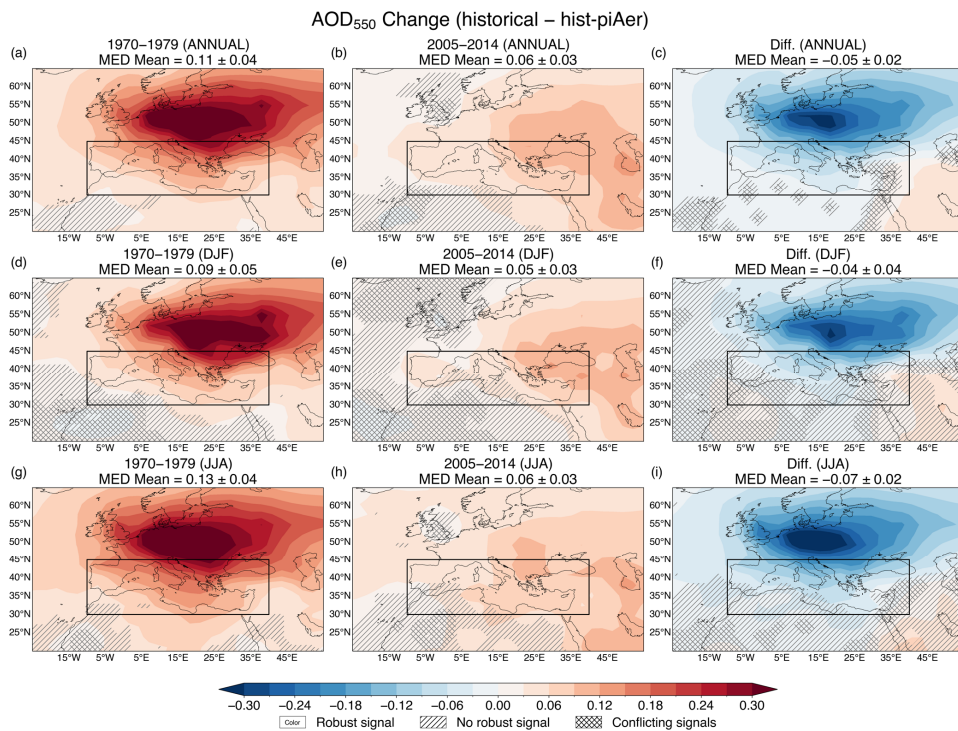
Figure 2. Changes in AOD due to anthropogenic aerosols over the Mediterranean (calculated from the difference historical minus hist-piAer ). Spatial patterns are presented for the periods 1970–1979 (left column), 2005–2014 (middle column) and their difference (2005–2014 minus 1970–1979; right column) on an annual scale (top row) and in boreal winter (DJF; middle row) and summer (JJA; bottom row). The multi-model ensemble means over the Mediterranean region (shown as a box) are shown along with the inter-model variability (one standard deviation) at the top of each panel. Colored areas without markings indicate robust changes, while hatched (/) and cross-hatched (X) areas indicate non-robust changes and conflicting signals, respectively.
