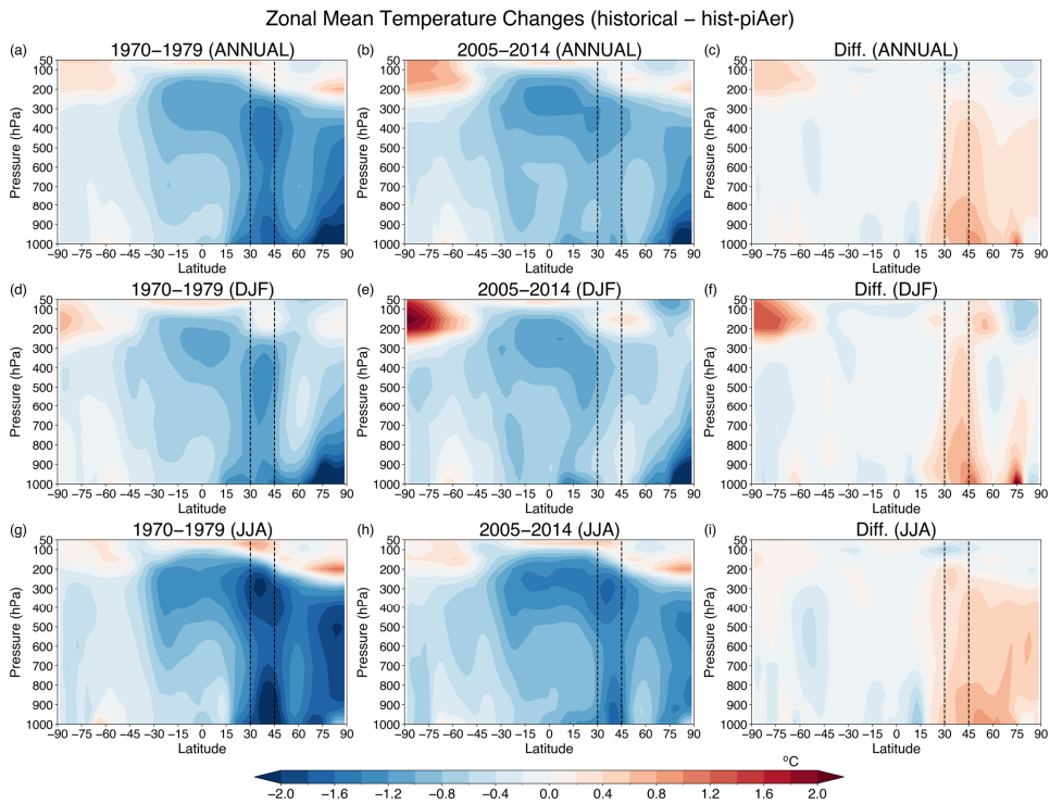
Figure 8. Changes in zonal mean temperature due to AAs (calculated from the difference historical minus hist-piAer ) for the MED longitudes (10°W – 40°E). Cross sections (pressure level over latitude) are presented for the periods 1970–1979 (left column), 2005–2014 (middle column) and their difference (2005–2014 minus 1970–1979; right column) on an annual scale (top row) and in boreal winter (DJF; middle row) and summer (JJA; bottom row). Dashed vertical lines indicate the latitudinal boundaries of the MED region.
