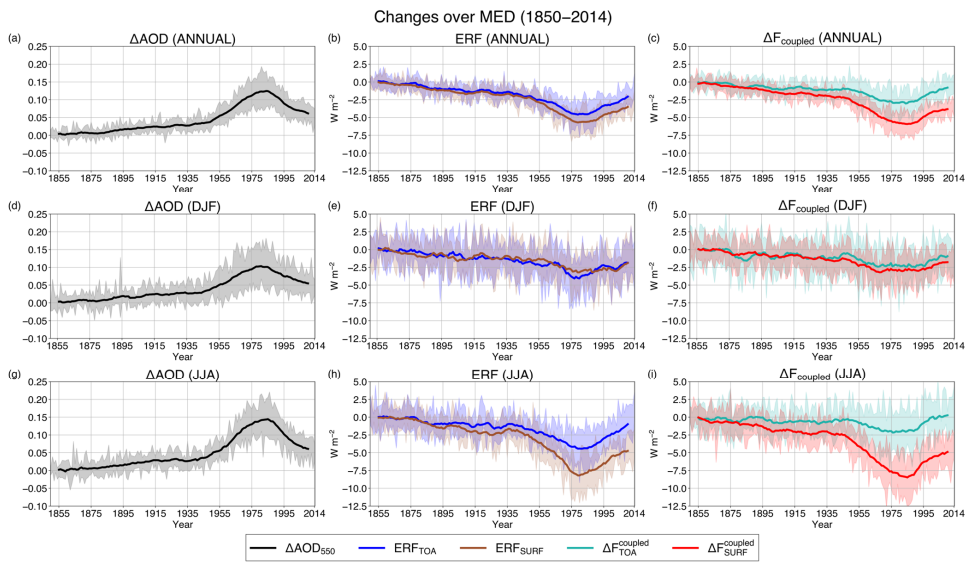
Figure 1. Timeseries of the AA-induced evolution of aerosol optical depth ( \Delta AOD ; left column), effective radiative forcing (ERF; middle column), and atmospheric radiative cooling at the surface ( \Delta F_{coupled} ; right column) over the Mediterranean region ( 10^{\circ}W-40^{\circ}E , 30^{\circ}N-45^{\circ}N ) for the historical period (1850–2014) on an annual scale (top row) and in boreal winter (DJF; middle row) and summer (JJA; bottom row). Changes in AOD and \Delta F_{coupled} were calculated from the difference historical minus hist-piAer , whereas ERF from the difference histSST minus histSST-piAer . The thin lines represent the annual weighted mean values, while thick lines represent the 10-year moving average, while shading expresses the inter-model variability (one standard deviation).
