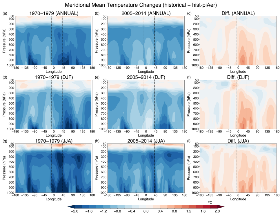
Figure 9. Changes in meridional mean temperature due to AAs (calculated from the difference historical minus hist-piAer ) for the MED latitudes (30°N – 45°N). Cross sections (pressure level over longitude) are presented for the periods 1970–1979 (left column), 2005–2014 (middle column) and their difference (2005–2014 minus 1970–1979; right column) on an annual scale (top row) and in boreal winter (DJF; middle row) and summer (JJA; bottom row). Dashed vertical lines indicate the longitudinal boundaries of the MED region.
