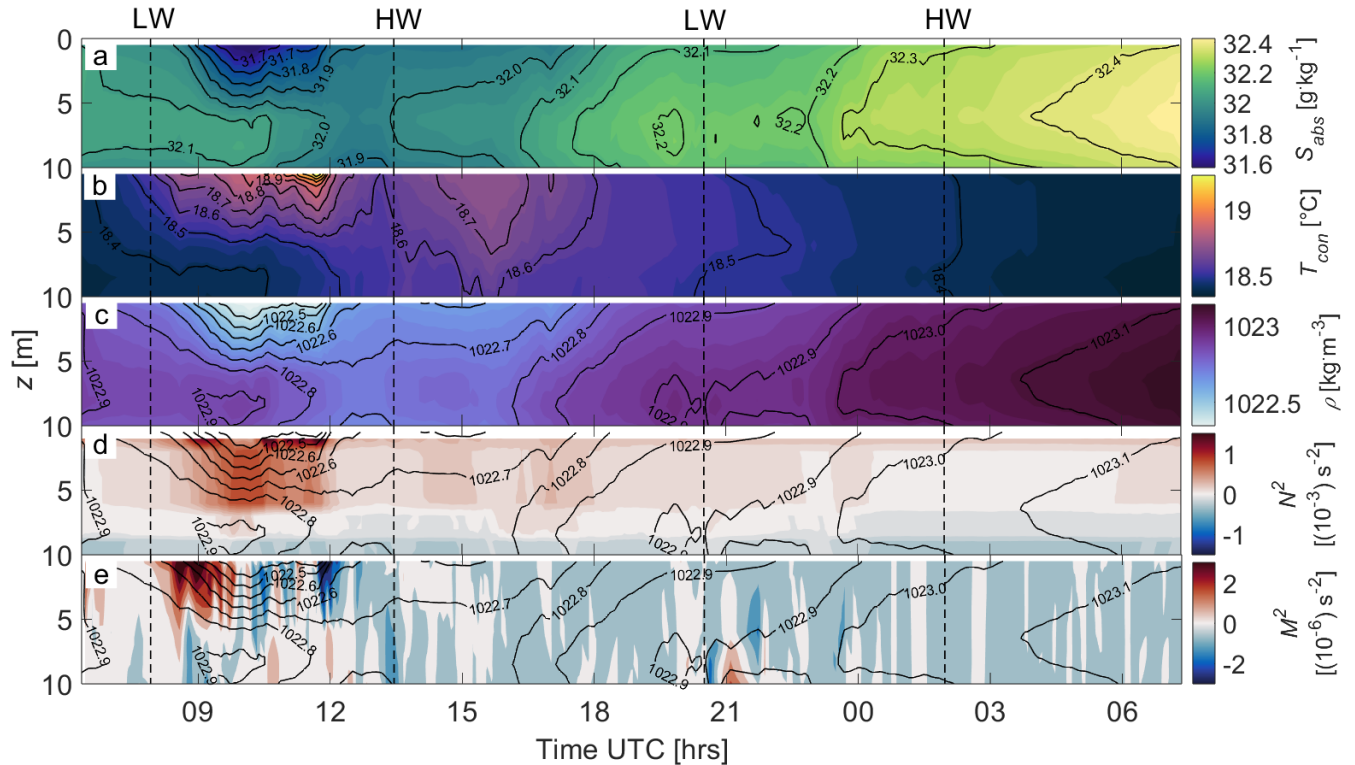
Figure 2. Time series of a) absolute salinity, b) conservative temperature, c) potential density, d) Brunt-Väissälä frequency N^2 and e) lateral buoyancy gradient M^2 obtained from the drifting sensor chain during August 5th and 6th. Vertical black dashed lines mark low water (LW) and high water (HW). N^2 and M^2 are displayed with overlain isopycnals. The low-density filament can be observed between the first LW and HW.
