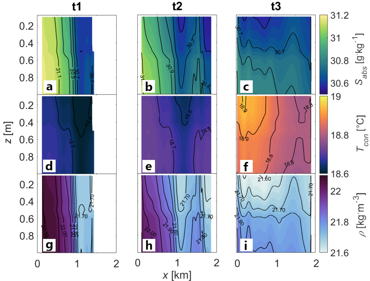
360 Figure 5. CTD data from the ASV displayed as contour section over depth across the filament at t1 = 07:23 am, t2 = 07:40 am and t3 = 08:30 am, each for of a-c) absolute salinity, d-f) conservative temperature and g-i) potential density in the upper NSL.
