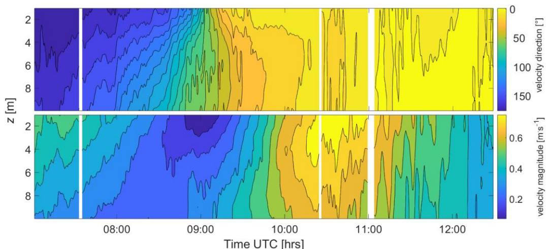
Figure E1. Contour of velocity magnitude and direction for August 5th over time and depth.
