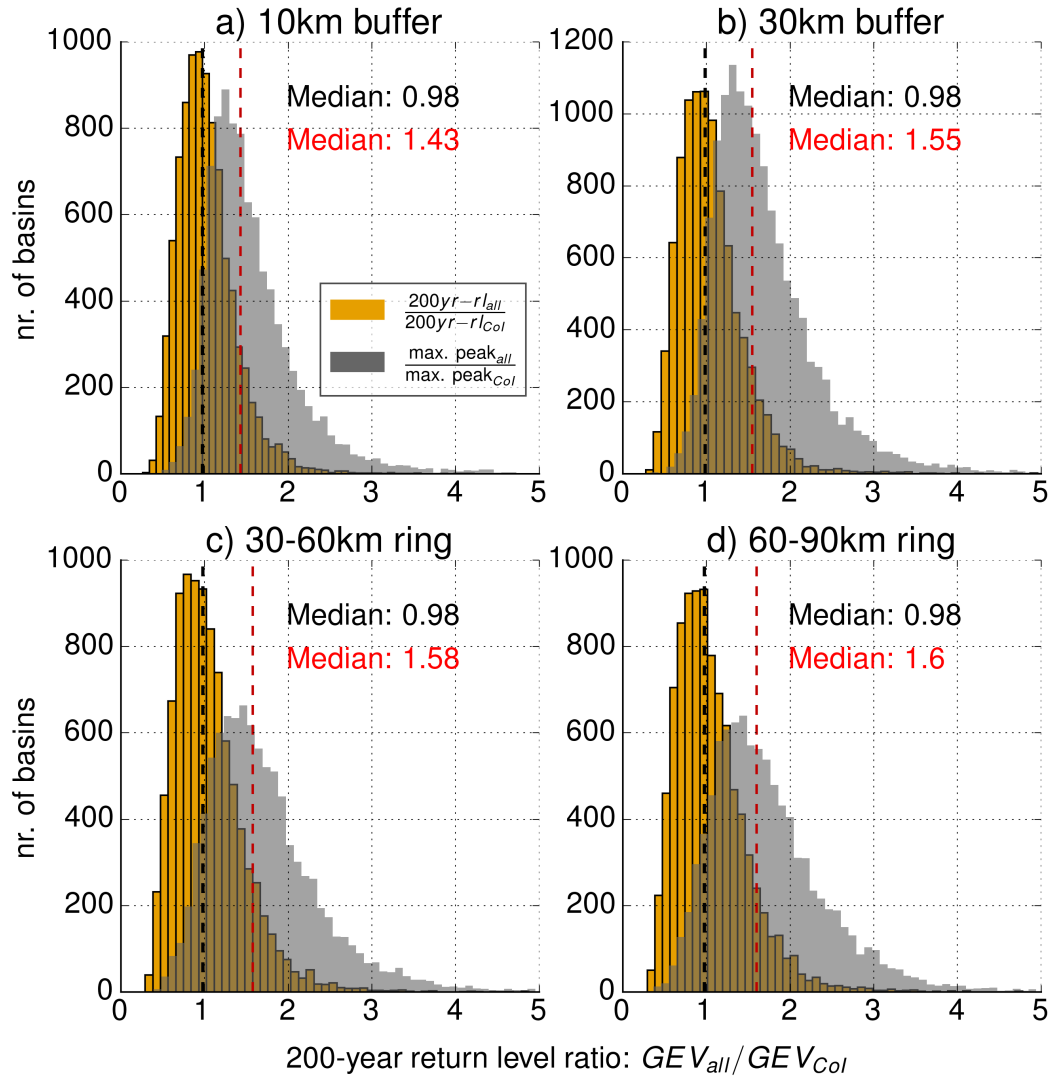
Figure 3. Histogram of the ratio between the 200-year return level from GEV_{all} and from GEV_{CoI} for four TDs. Gray histograms indicate the ratio of the highest peaks in the respective datasets used for fitting (see main text for further explanation). The median ratio of the return levels ratio is marked in black, and the median ratio of maximum peak discharge values in red.
