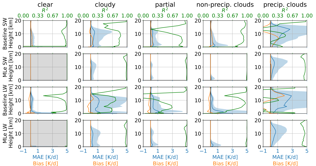
Figure 4. Comparison of the baseline and the ML-enhanced radiation scheme on coarse-grained QUBICC data. Results are shown for the shortwave (top rows) and longwave (bottom rows) spectral range. The results are shown separately for clear-sky samples (no clouds, left column), fully cloudy sky samples (second column), and samples with partial cloudiness (third column). Additionally, the results are separated by non-precipitating (fourth column) and precipitating clouds (fifth column). The shown metrics are coefficient of determination R^2 (green), bias (orange) and MAE (blue) with 95% of the spread, which is defined as the spread between the 2.5% percentile and the 97.5% percentiles. The bias and MAE share the x-axis. The ML-clear-sky panels are gray because the clear-sky fluxes are not calculated by the ML model, but shown as reference.
