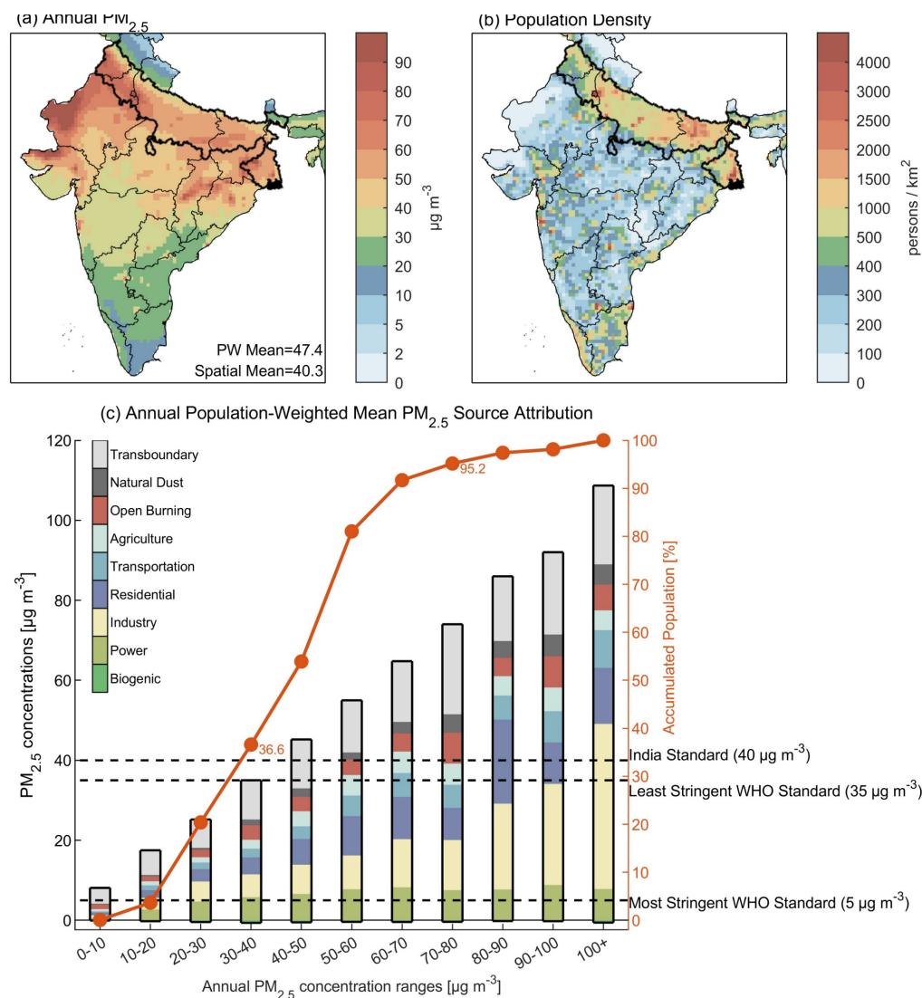
Figure 5. Baseline annual PM_{2.5} concentrations in 2022 across India and their source attribution. In a , Annual results are calculated as the average of January, April, July, and October simulations. Spatial distribution of annual average PM_{2.5} concentrations across India are shown in color. National averages for Population-Weighted (PW) and spatial mean PM_{2.5} concentrations are given as inset values in the figure. Panel b shows gridded population density across India. In a and b , the thick black line denotes the boundary of the Indo-Gangetic Plain (IGP). In c , WRF-Chem grids are aggregated by ranges of annual mean PM_{2.5} concentrations, with colored bars indicating source attribution (left Y axis). The red line and dots indicate the cumulative percentage of the population (right Y axis) living in areas where the annual mean PM_{2.5} concentration falls within or below a given concentration range. For example, 36.6% (95.2%) of the Indian population was exposed to annual PM_{2.5} concentrations < 40 (80) \mu g/m^3 in 2022. See monthly versions of panel c in Supplementary Figure 5 .
