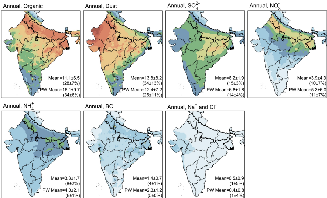
690 Figure 8. Spatial pattern of annual concentrations of \text{PM}_{2.5} components across India in 2022. Annual results are calculated as the average of January, April, July, and October simulations. In each panel, numbers outside parentheses
