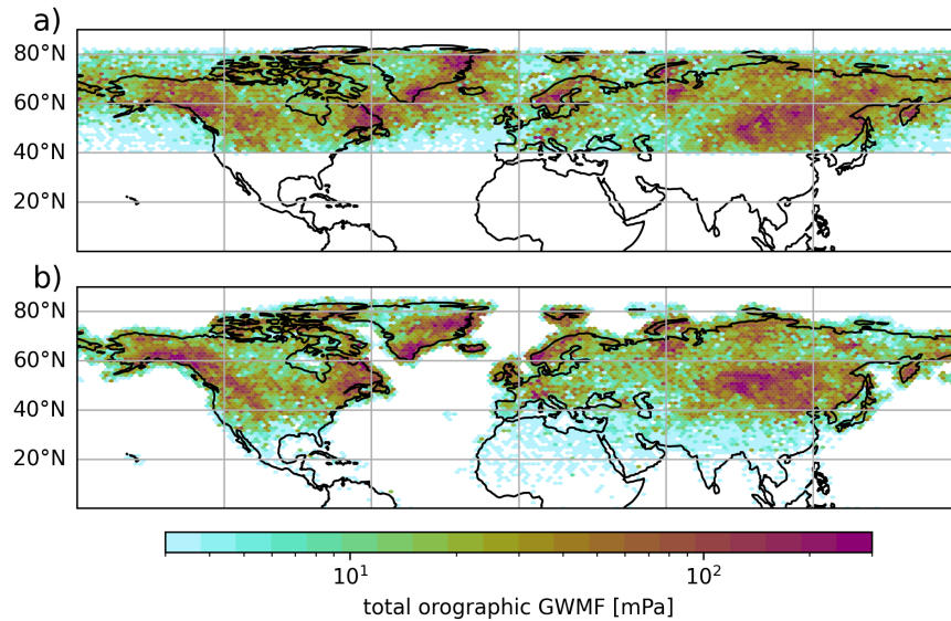
Figure B1. Same as Fig. 6 but for the period 2019-12-10 to 2020-03-31. Top: simulated observations of orographic GWs at 35 km altitude; bottom: backtraced source location for all observed MWs.
