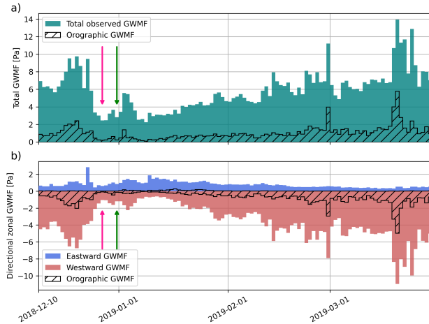
Figure 3. Timeline-Time series of observed GWMF at 35 km altitude north of 40°N during the unfolding of the SSW (SSW onset on 31st December, Rao et al. (2019)). Panel a) shows the total absolute GWMF, panel b) the zonal GWMF summed for eastward and westward directions separately. The part of the observed GWMF that can be attributed to orographic sources is shown with hatching in both panels. The pink and green arrows point at the time of the wind reversal at 35 km and the central SSW date, respectively.
