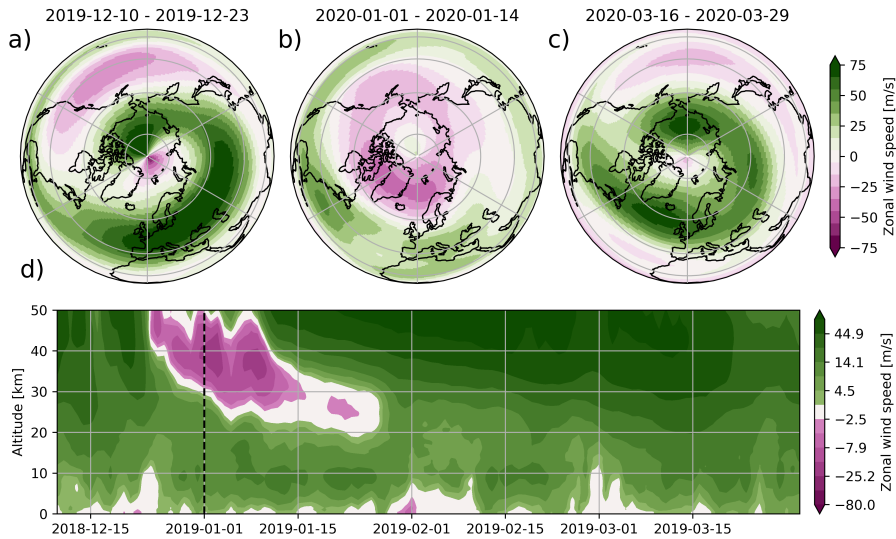
Figure 4. Wind situation during the SSW. Panels a-c show two-week averaged zonal wind speed at 35 km altitude before, during, and after the SSW. Panel d shows the time-altitude cross section of zonal mean zonal wind at 60° N.
