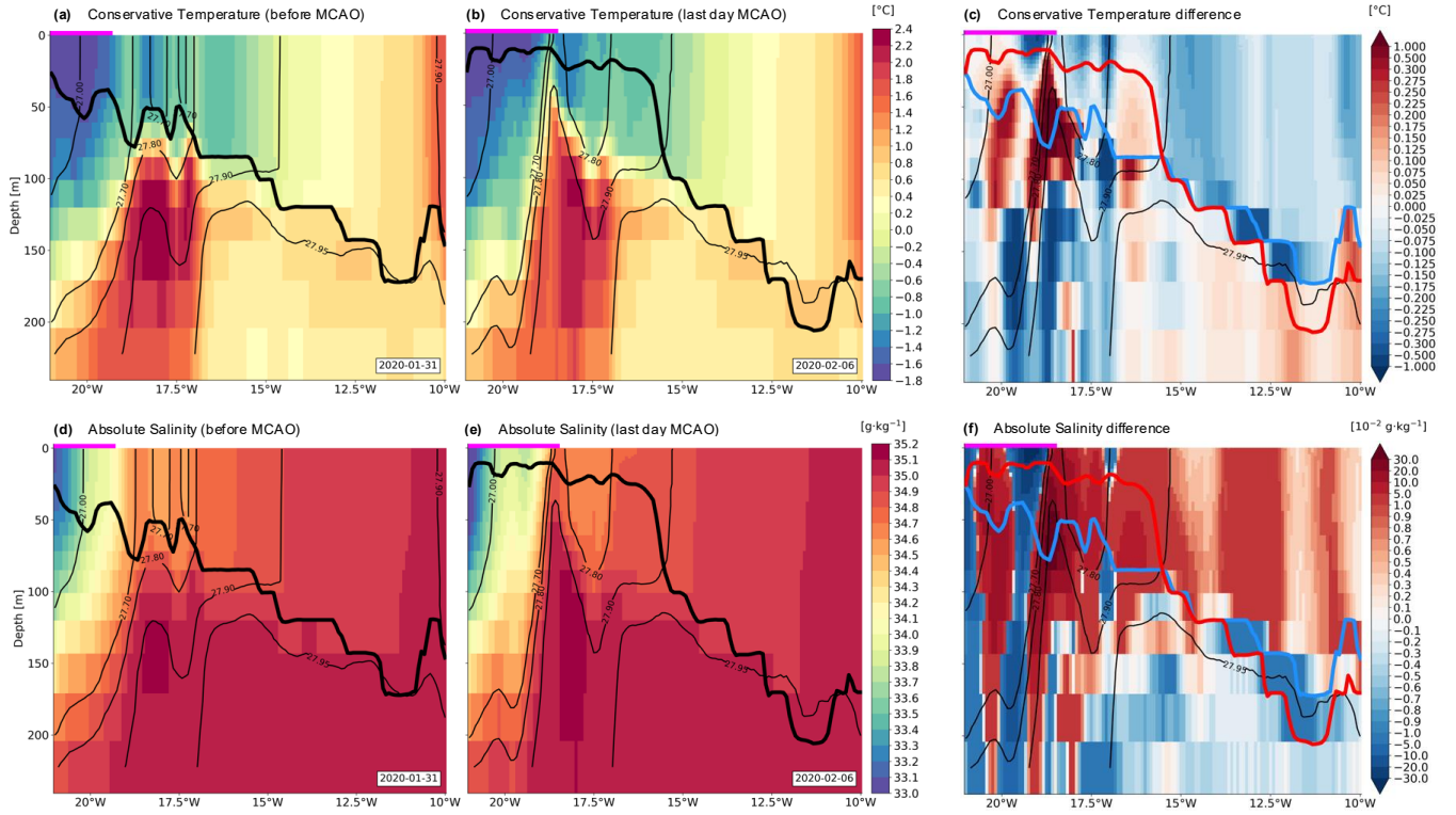
Figure 7. Vertical cross-sections at 71^{\circ}\text{N} in the Iceland Sea (cf. black line in Fig. 1). (a) Conservative Temperature ( ^{\circ}\text{C} ) before the MCAO (31/01/2020), (b) during the last day (06/02/2020) and (c) their difference. (d) Absolute Salinity ( \text{g}\cdot\text{kg}^{-1} ) before the MCAO (31/01/2020), (e) during the last day (06/02/2020) and (f) their difference. Note the non-linear scale in panels (c) and (f). The thin black contours in panels (a), (b), (d), and (e) correspond to the density contours on the considered day, while in (c) and (f) they correspond to the density contours during the last day (06/02/2020). The thick black lines in panels (a), (b), (d), and (e) indicate the mixed-layer depth on the considered day, while thick blue and red lines in panels (c) and (f) indicate the mixed-layer depth before the MCAO (31/01/2020) and during the last day (06/02/2020), respectively. The magenta lines indicate areas where the ocean surface is covered by at least 15 % sea ice concentration during the considered day in panels (a), (b), (d), (e), and during the last day in (c) and (f).
