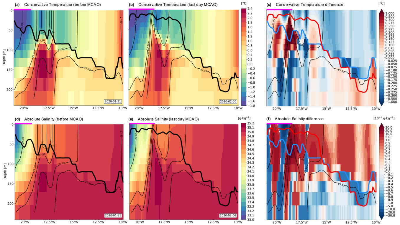
Figure 7. Vertical cross-sections at 71^\circ\text{N} in the Iceland Sea (cf. black line in Fig. 1). (a) Conservative Temperature ( ^\circ\text{C} ) before the MCAO (31/01/2020), (b) during the last day (06/02/2020) and (c) their difference. (d) Absolute Salinity ( \text{g}\cdot\text{kg}^{-1} ) before the MCAO (31/01/2020), (e) during the last day (06/02/2020) and (f) their difference. Note the non-linear scale in panels (c) and (f). The thin black contours in panels (a), (b), (d), and (e) correspond to the density contours on the considered day, while in (c) and (f) they correspond to the density contours during the last day (06/02/2020). The thick black lines in panels (a), (b), (d), and (e) indicate the mixed-layer depth on the considered day, while thick blue and red lines in panels (c) and (f) indicate the mixed-layer depth before the MCAO (31/01/2020) and during the last day (06/02/2020), respectively. The magenta lines indicate areas where the ocean surface is covered by at least 15 % sea ice concentration during the considered day in panels (a), (b), (d), (e), and during the last day in (c) and (f).
