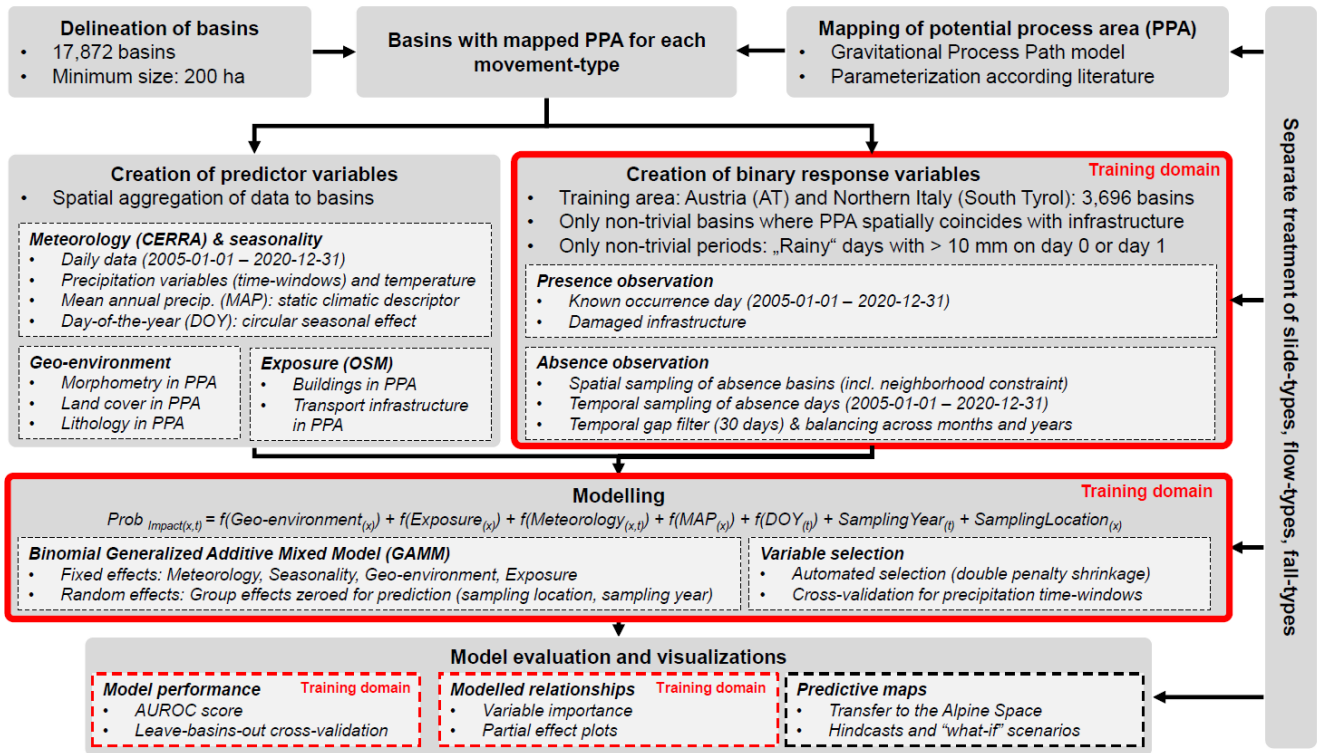
225 Figure 2: Methodical framework of this study. Aspects referring exclusively to the training domain (Austria, South Tyrol) are highlighted in red, while processing steps applied to the entire Alpine Space are shown without red borders.
