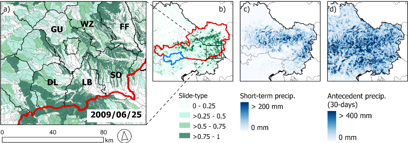
Figure 12: Hindcast example of a severe event in Styria, Austria. Model predictions from the slide-type model for June 25, 2009, are shown for the focus area of the event (a) and the calibration area of Austria (red in b) and South Tyrol (blue in b), together with the variables representing short-term precipitation (c) and 30-day antecedent precipitation (d). Black polygons in (a) delineate the districts of Styria, with labels showing the districts linked to the most private damage reports: Südoststeiermark (SO, 600 reports), Leibnitz (LB, 324), Weiz (WZ, 287), Graz-Umgebung (GU, 205), Deutschlandsberg (DL, 95) and Fürstenfeld (FF, 62) according to Hornich and Adelwöhrer (2010). Hindcast animations of this event are provided in the supplementary material (S7 at: https://doi.org/10.6084/m9.figshare.30271795.v1 ).
