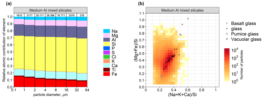
Figure 2. TSI (a) Average elemental composition (atomic fraction) as a function of particle size for the medium-Al mixed-silicate (MAS) particles at Dyngjúsandur from deposition plate and free-wing impactor samples. The numbers on top represent total particle counts in the given size bin. (b) Two-dimensional histogram with respect to element atomic concentration ratios for MAS particles. In addition, positions and classifications of particles identified manually by composition and morphology are shown.
