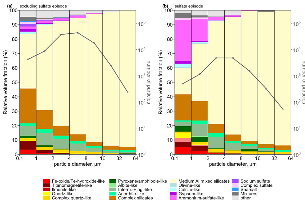
Figure 4. Size-resolved relative volume fraction of different particle groups at Dyngjúsandur, Iceland, in 2021. The curve shows the number of particles analyzed for each size bin. For simplification of display, several composition groups have been combined in this plot. “Complex silicates” consist of the following groups: complex silicate (high Al), complex silicate (moderate Al–low alkali), Al-rich clay mineral, other silicate, and Ca-rich silicate / Ca–Si mixture. “Mixtures” comprise the following groups: sea-salt / silicate mixture, aged-sea-salt / silicate mixture, sodium sulfate / silicate mixture, sulfate / silicate mixture, and complex mixture. For details on the classification scheme, refer to Supplement S3 TS2 .
