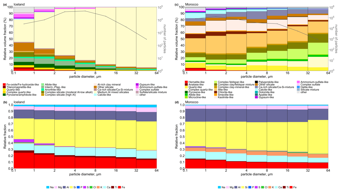
Figure 9. Size-resolved elemental and mineralogical composition for Icelandic (a,b) and Moroccan (c,d) dust, respectively.
